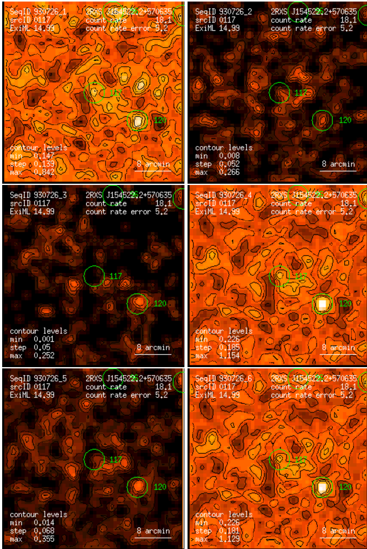
Figure 117: RASS 930726: detection 0117: band rate images, Gaussian filter: (1) PSPC channels 11 – 41, (2) 52 – 90, (3) 91 – 201, (4) 11 – 235, (5) 52 – 201, (6) 11 – 201. Broad band rates in counts/ks. Band rate contour levels in counts/ks/arcmin 2 .
