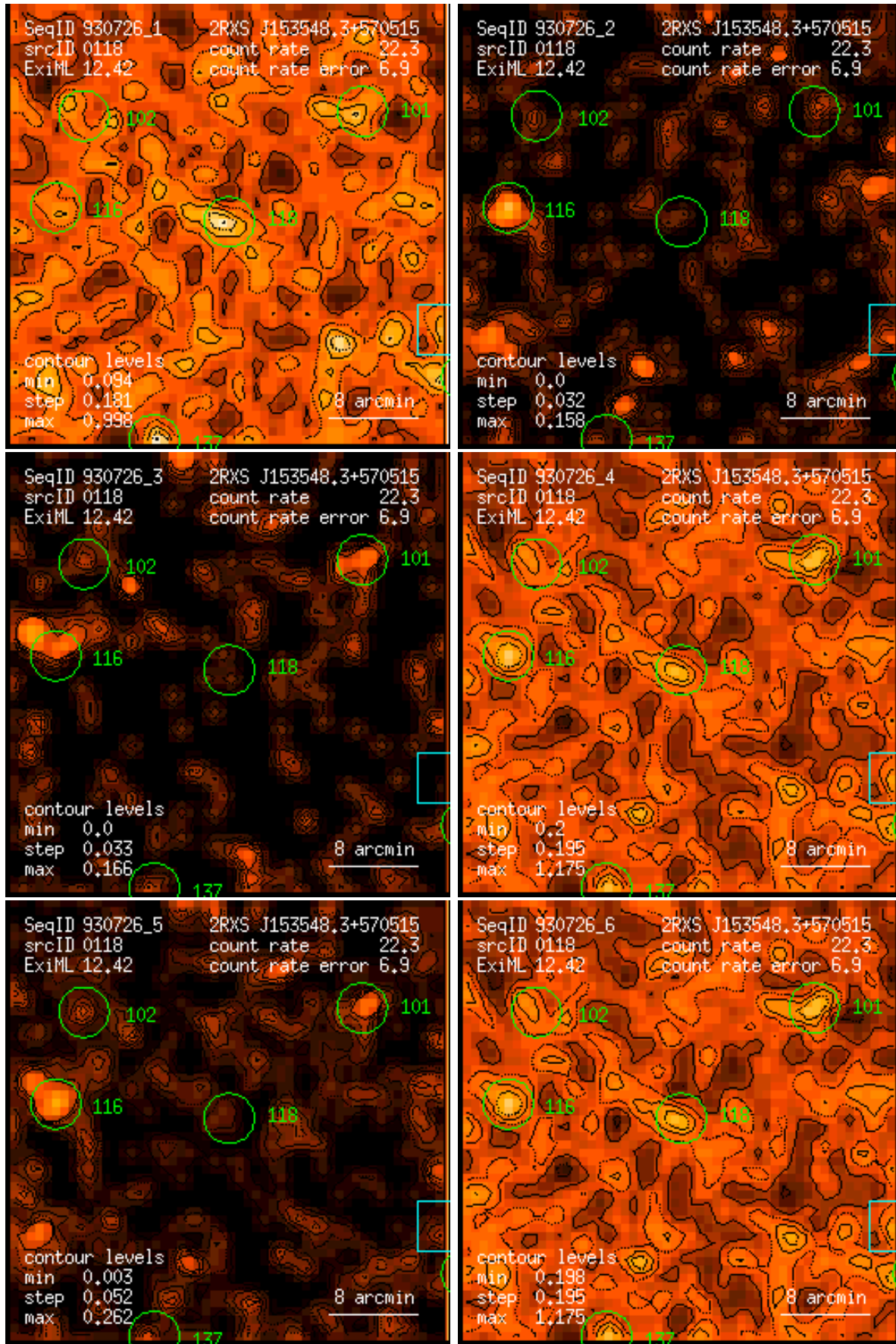
Figure 118: RASS 930726: detection 0118: band rate images, Gaussian filter: (1) PSPC channels 11 – 41, (2) 52 – 90, (3) 91 – 201, (4) 11 – 235, (5) 52 – 201, (6) 11 – 201. Broad band rates in counts/ks. Band rate contour levels in counts/ks/arcmin 2 .
