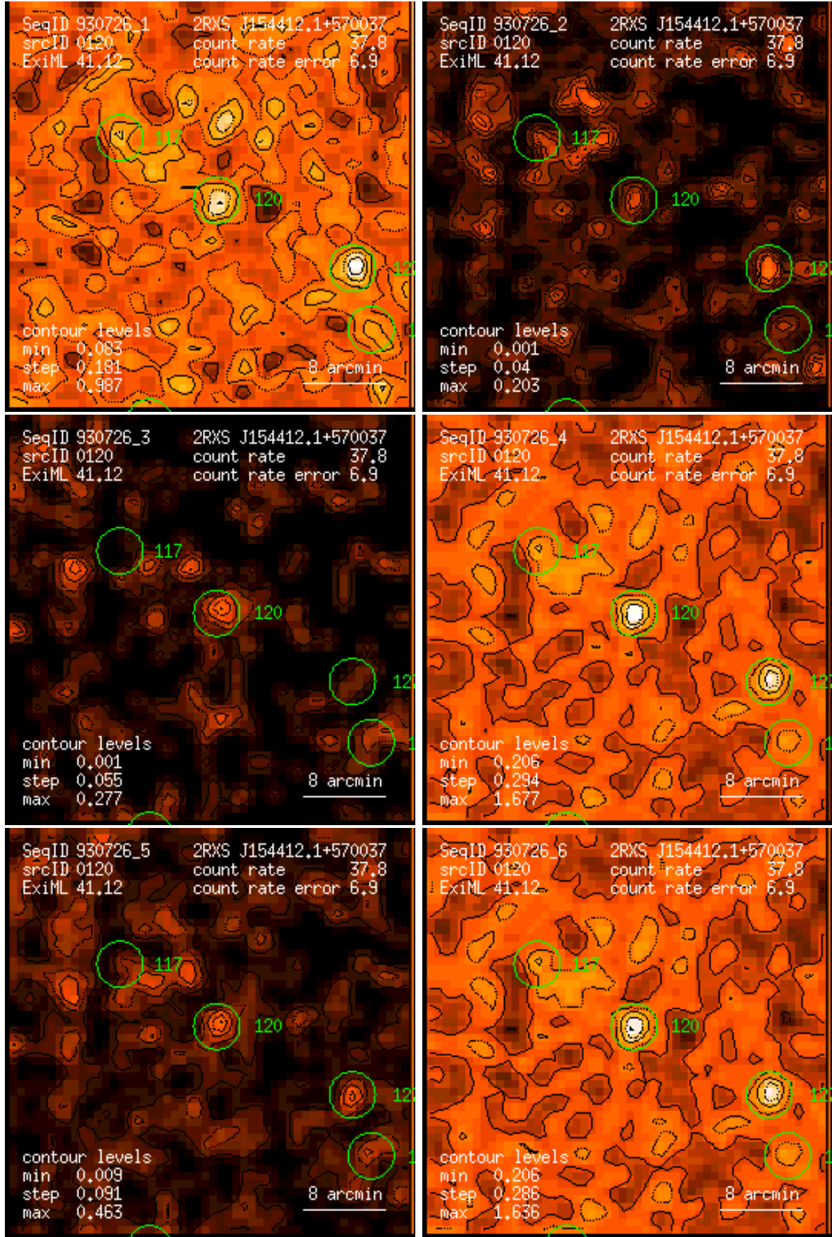
Figure 120: RASS 930726: detection 0120: band rate images, Gaussian filter: (1) PSPC channels 11 – 41, (2) 52 – 90, (3) 91 – 201, (4) 11 – 235, (5) 52 – 201, (6) 11 – 201. Broad band rates in counts/ks. Band rate contour levels in counts/ks/arcmin 2 .
