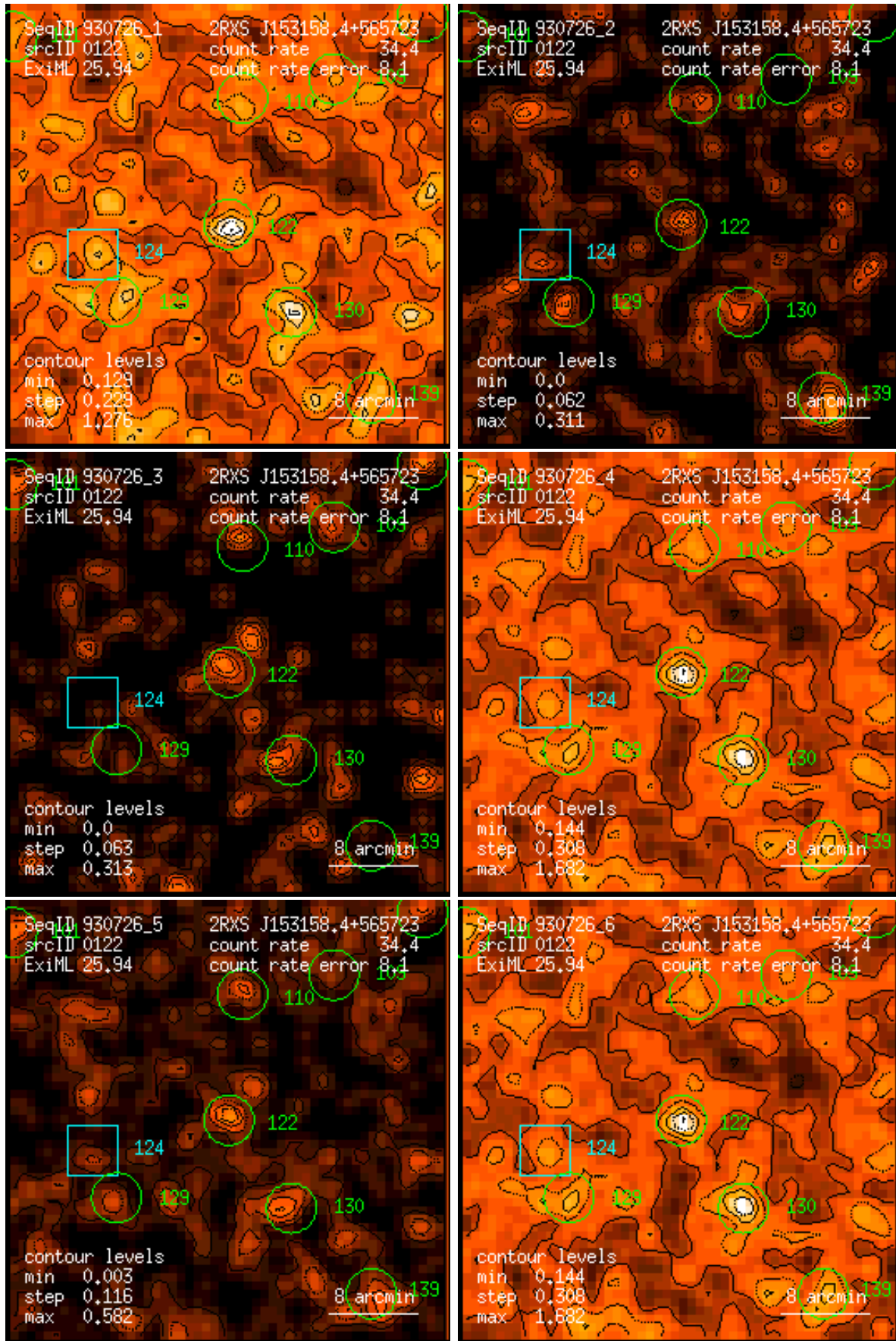
Figure 122: RASS 930726: detection 0122: band rate images, Gaussian filter: (1) PSPC channels 11 – 41, (2) 52 – 90, (3) 91 – 201, (4) 11 – 235, (5) 52 – 201, (6) 11 – 201. Broad band rates in counts/ks. Band rate contour levels in counts/ks/arcmin 2 .
