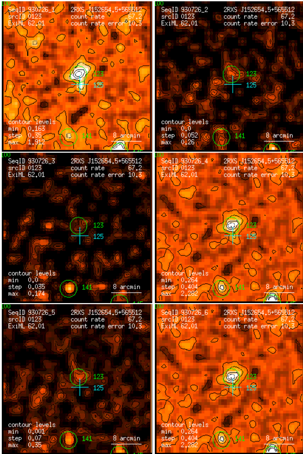
Figure 123: RASS 930726: detection 0123: band rate images, Gaussian filter: (1) PSPC channels 11 – 41, (2) 52 – 90, (3) 91 – 201, (4) 11 – 235, (5) 52 – 201, (6) 11 – 201. Broad band rates in counts/ks. Band rate contour levels in counts/ks/arcmin 2 .
