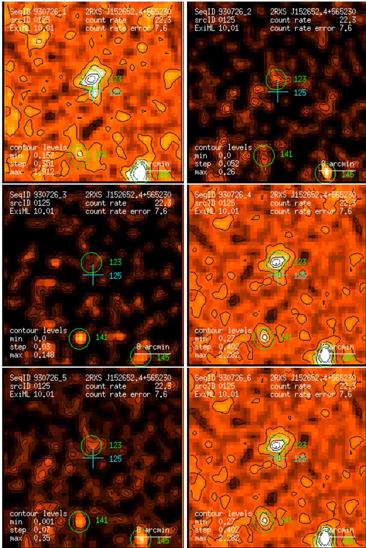
Figure 125: RASS 930726: detection 0125: band rate images, Gaussian filter: (1) PSPC channels 11 – 41, (2) 52 – 90, (3) 91 – 201, (4) 11 – 235, (5) 52 – 201, (6) 11 – 201. Broad band rates in counts/ks. Band rate contour levels in counts/ks/arcmin 2 .
