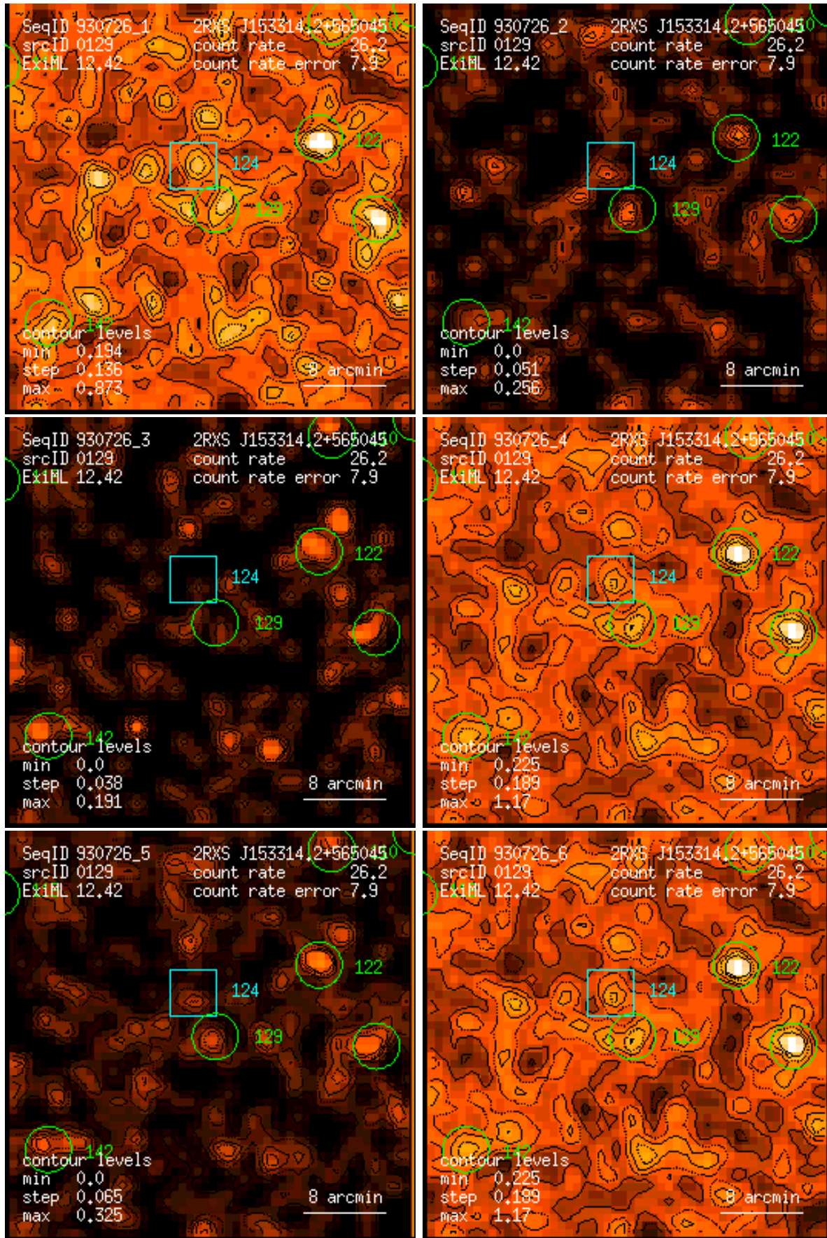
Figure 129: RASS 930726: detection 0129: band rate images, Gaussian filter: (1) PSPC channels 11 – 41, (2) 52 – 90, (3) 91 – 201, (4) 11 – 235, (5) 52 – 201, (6) 11 – 201. Broad band rates in counts/ks. Band rate contour levels in counts/ks/arcmin 2 .
