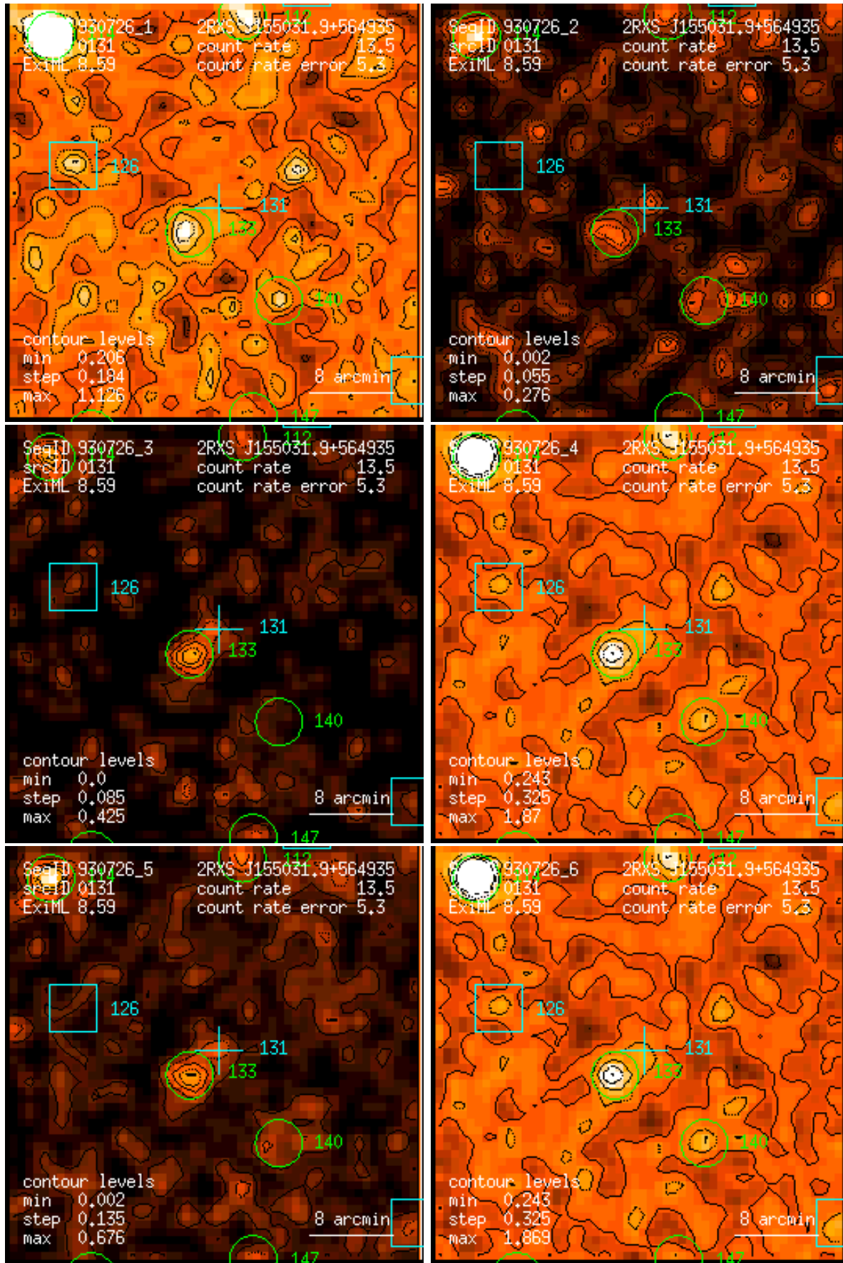
Figure 131: RASS 930726: detection 0131: band rate images, Gaussian filter: (1) PSPC channels 11 – 41, (2) 52 – 90, (3) 91 – 201, (4) 11 – 235, (5) 52 – 201, (6) 11 – 201. Broad band rates in counts/ks. Band rate contour levels in counts/ks/arcmin 2 .
