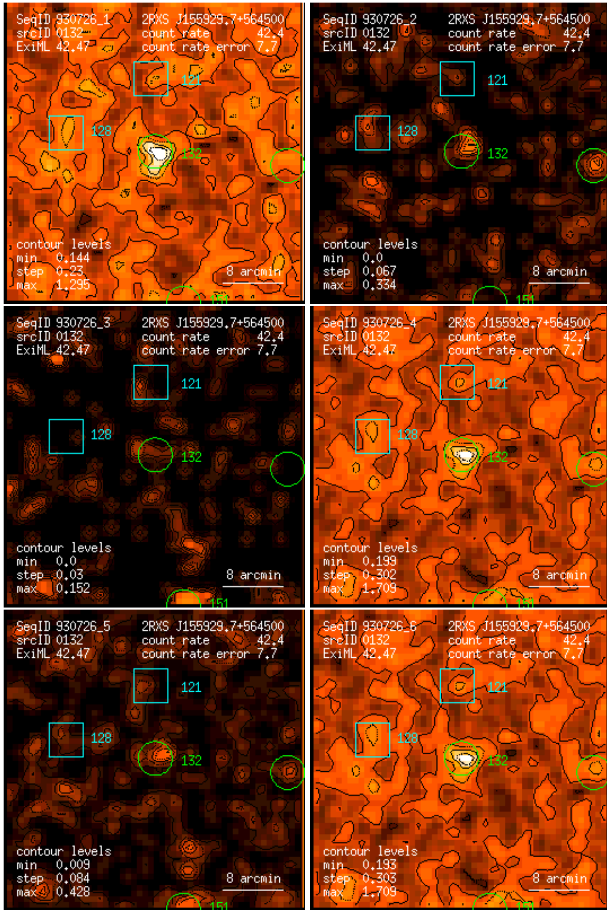
Figure 132: RASS 930726: detection 0132: band rate images, Gaussian filter: (1) PSPC channels 11 – 41, (2) 52 – 90, (3) 91 – 201, (4) 11 – 235, (5) 52 – 201, (6) 11 – 201. Broad band rates in counts/ks. Band rate contour levels in counts/ks/arcmin 2 .
