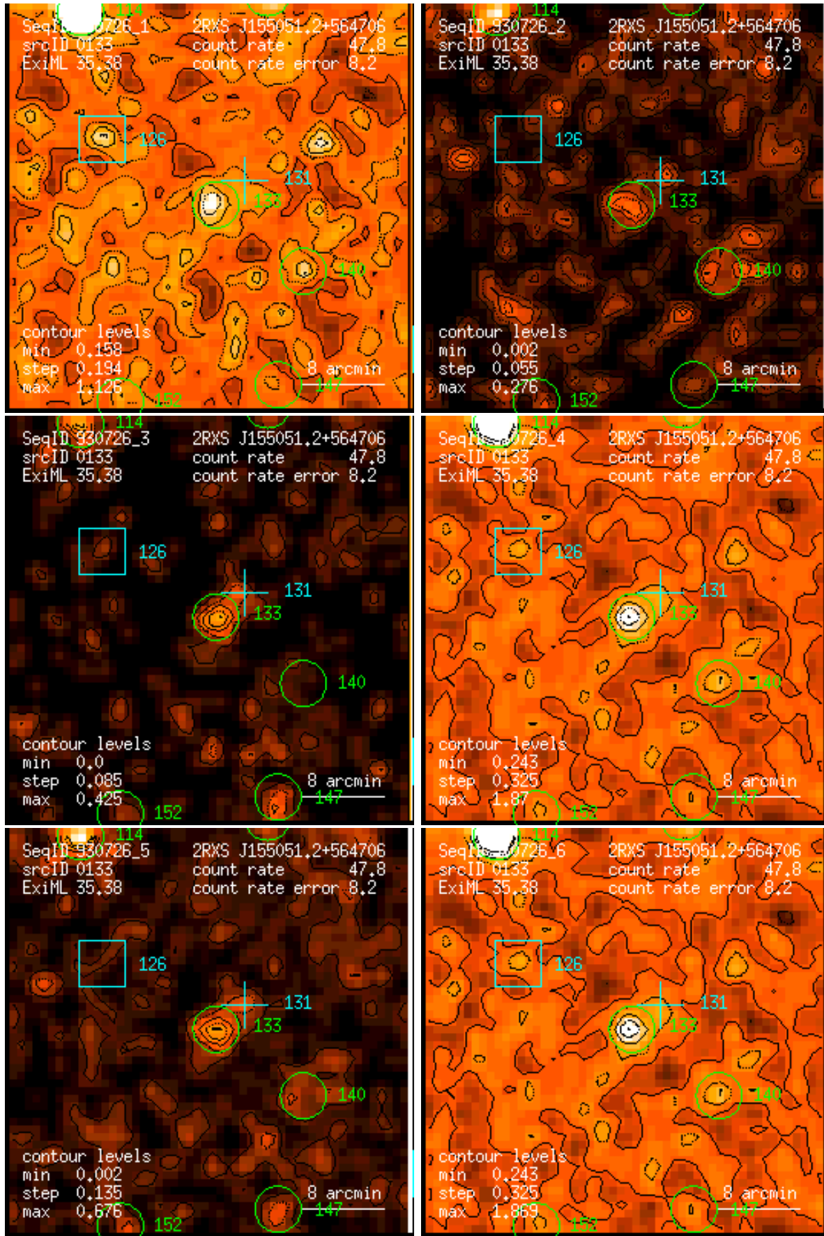
Figure 133: RASS 930726: detection 0133: band rate images, Gaussian filter: (1) PSPC channels 11 – 41, (2) 52 – 90, (3) 91 – 201, (4) 11 – 235, (5) 52 – 201, (6) 11 – 201. Broad band rates in counts/ks. Band rate contour levels in counts/ks/arcmin 2 .
