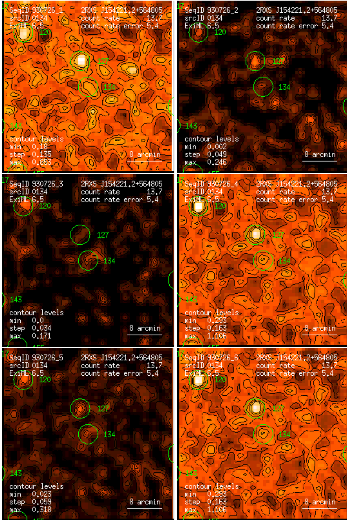
Figure 134: RASS 930726: detection 0134: band rate images, Gaussian filter: (1) PSPC channels 11 – 41, (2) 52 – 90, (3) 91 – 201, (4) 11 – 235, (5) 52 – 201, (6) 11 – 201. Broad band rates in counts/ks. Band rate contour levels in counts/ks/arcmin 2 .
