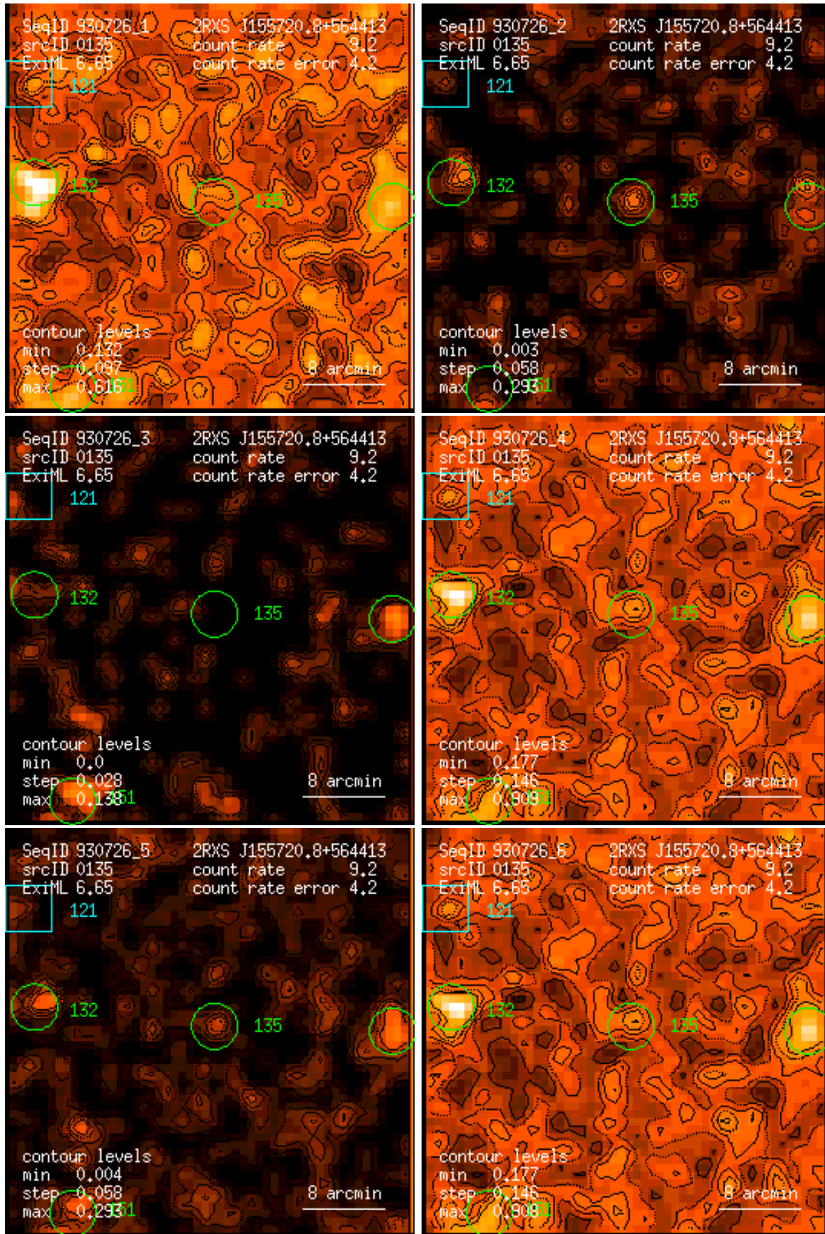
Figure 135: RASS 930726: detection 0135: band rate images, Gaussian filter: (1) PSPC channels 11 – 41, (2) 52 – 90, (3) 91 – 201, (4) 11 – 235, (5) 52 – 201, (6) 11 – 201. Broad band rates in counts/ks. Band rate contour levels in counts/ks/arcmin 2 .
