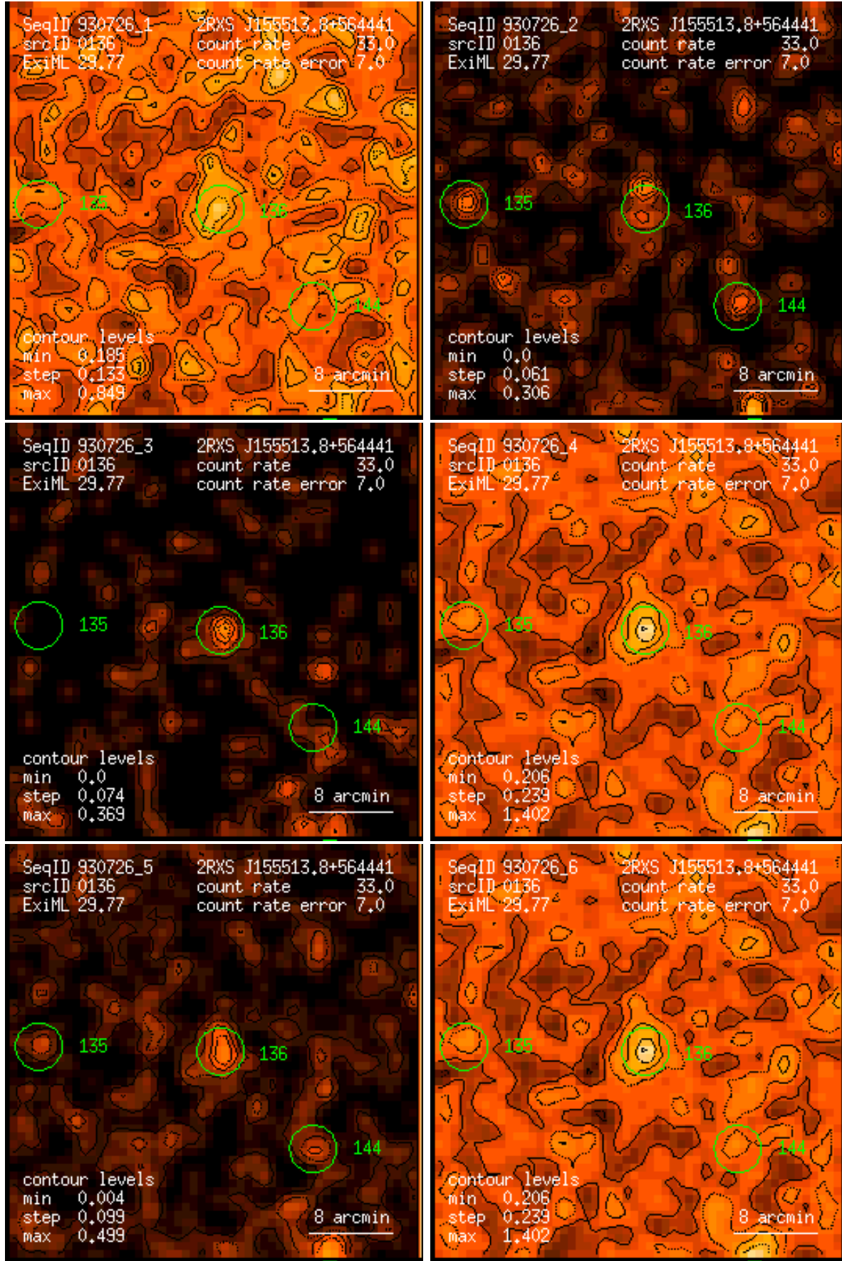
Figure 136: RASS 930726: detection 0136: band rate images, Gaussian filter: (1) PSPC channels 11 – 41, (2) 52 – 90, (3) 91 – 201, (4) 11 – 235, (5) 52 – 201, (6) 11 – 201. Broad band rates in counts/ks. Band rate contour levels in counts/ks/arcmin 2 .
