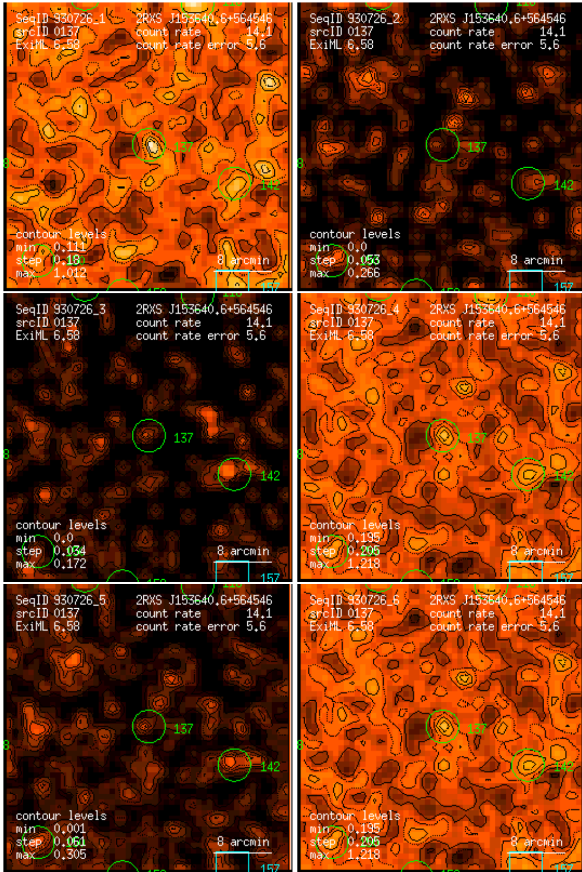
Figure 137: RASS 930726: detection 0137: band rate images, Gaussian filter: (1) PSPC channels 11 – 41, (2) 52 – 90, (3) 91 – 201, (4) 11 – 235, (5) 52 – 201, (6) 11 – 201. Broad band rates in counts/ks. Band rate contour levels in counts/ks/arcmin 2 .
