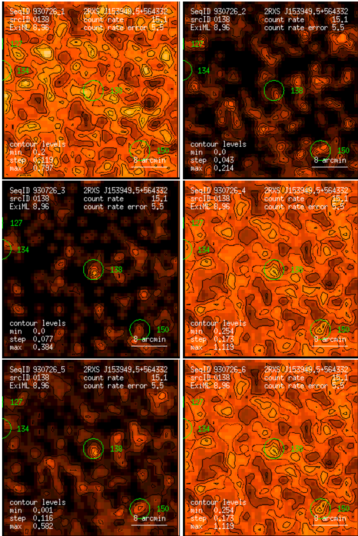
Figure 138: RASS 930726: detection 0138: band rate images, Gaussian filter: (1) PSPC channels 11 – 41, (2) 52 – 90, (3) 91 – 201, (4) 11 – 235, (5) 52 – 201, (6) 11 – 201. Broad band rates in counts/ks. Band rate contour levels in counts/ks/arcmin 2 .
