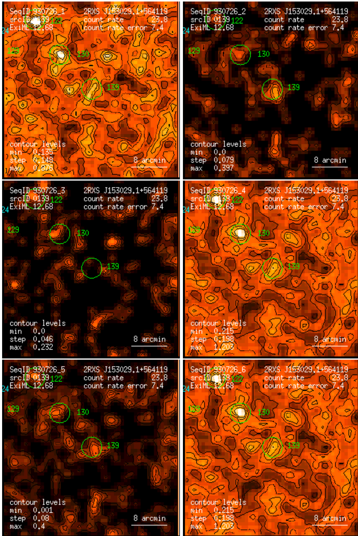
Figure 139: RASS 930726: detection 0139: band rate images, Gaussian filter: (1) PSPC channels 11 – 41, (2) 52 – 90, (3) 91 – 201, (4) 11 – 235, (5) 52 – 201, (6) 11 – 201. Broad band rates in counts/ks. Band rate contour levels in counts/ks/arcmin 2 .
