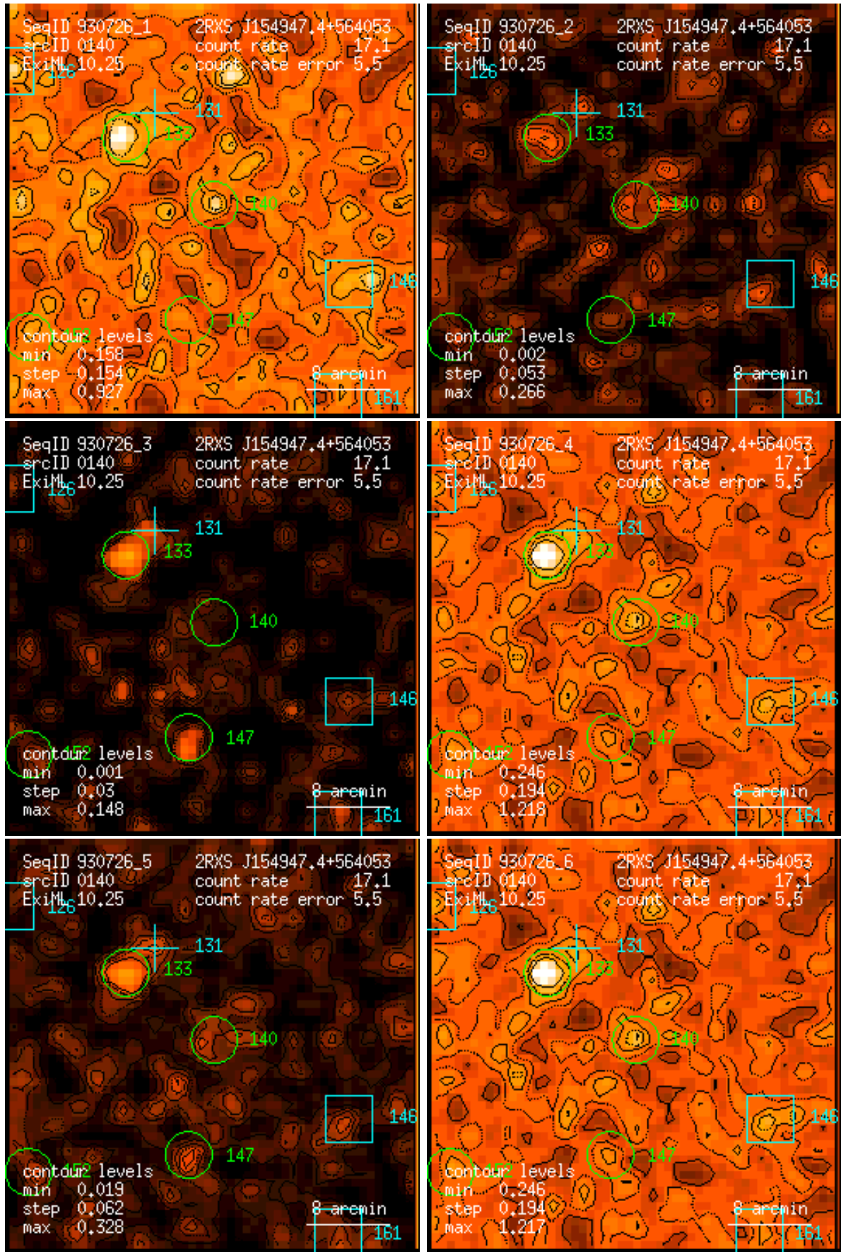
Figure 140: RASS 930726: detection 0140: band rate images, Gaussian filter: (1) PSPC channels 11 – 41, (2) 52 – 90, (3) 91 – 201, (4) 11 – 235, (5) 52 – 201, (6) 11 – 201. Broad band rates in counts/ks. Band rate contour levels in counts/ks/arcmin 2 .
