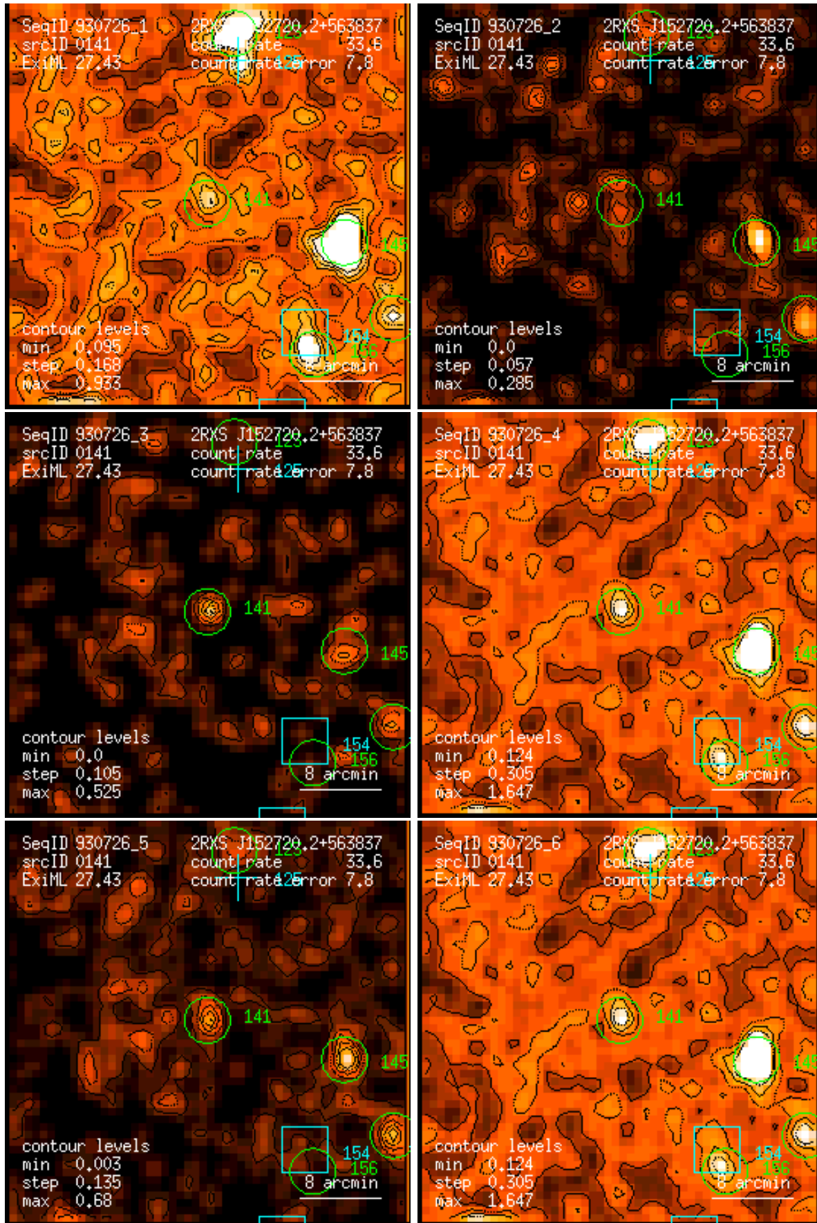
Figure 141: RASS 930726: detection 0141: band rate images, Gaussian filter: (1) PSPC channels 11 – 41, (2) 52 – 90, (3) 91 – 201, (4) 11 – 235, (5) 52 – 201, (6) 11 – 201. Broad band rates in counts/ks. Band rate contour levels in counts/ks/arcmin 2 .
