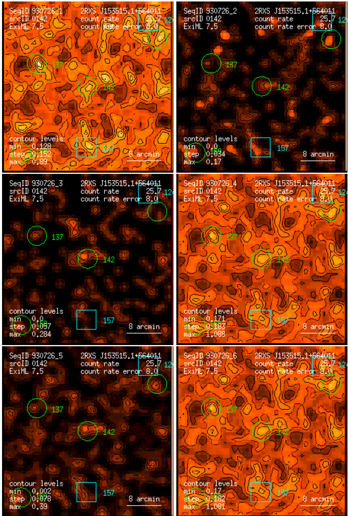
Figure 142: RASS 930726: detection 0142: band rate images, Gaussian filter: (1) PSPC channels 11 – 41, (2) 52 – 90, (3) 91 – 201, (4) 11 – 235, (5) 52 – 201, (6) 11 – 201. Broad band rates in counts/ks. Band rate contour levels in counts/ks/arcmin 2 .
