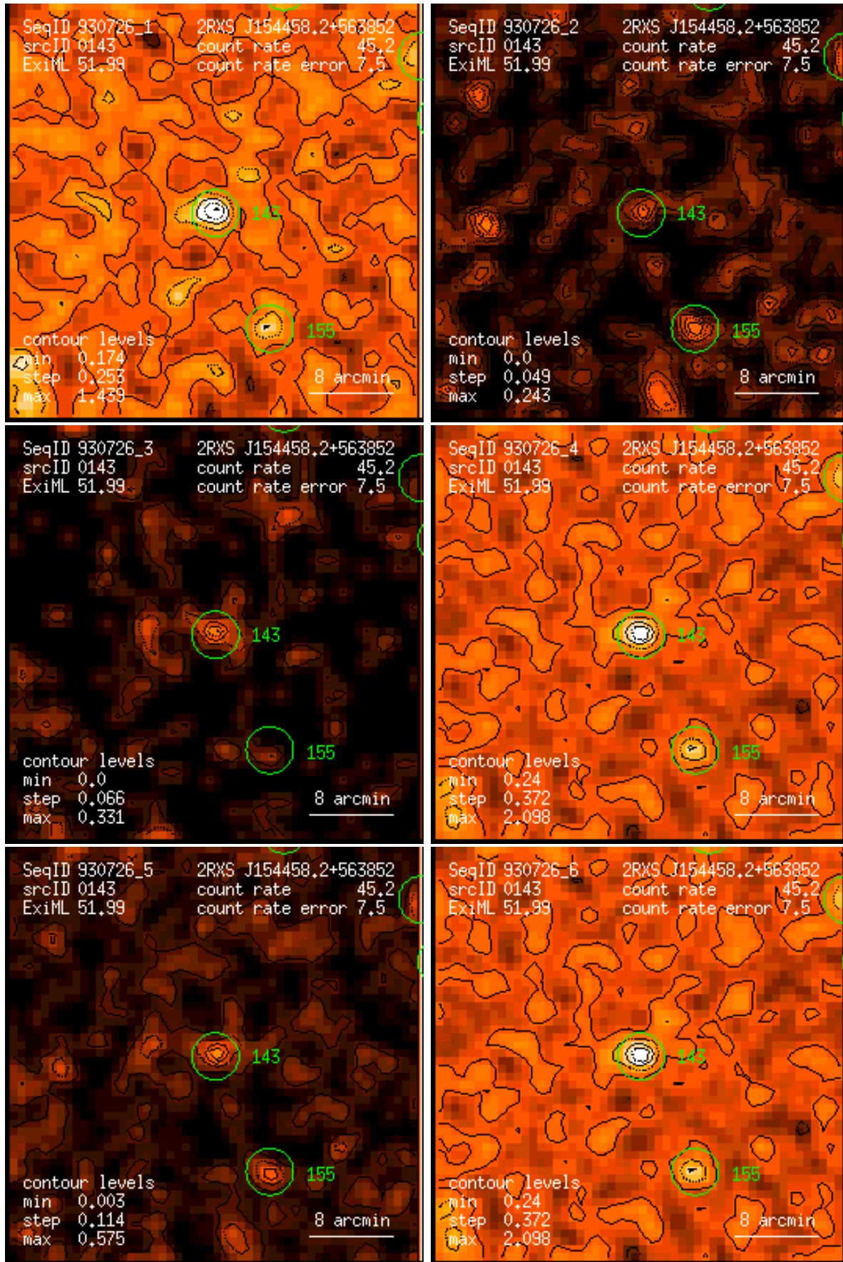
Figure 143: RASS 930726: detection 0143: band rate images, Gaussian filter: (1) PSPC channels 11 – 41, (2) 52 – 90, (3) 91 – 201, (4) 11 – 235, (5) 52 – 201, (6) 11 – 201. Broad band rates in counts/ks. Band rate contour levels in counts/ks/arcmin 2 .
