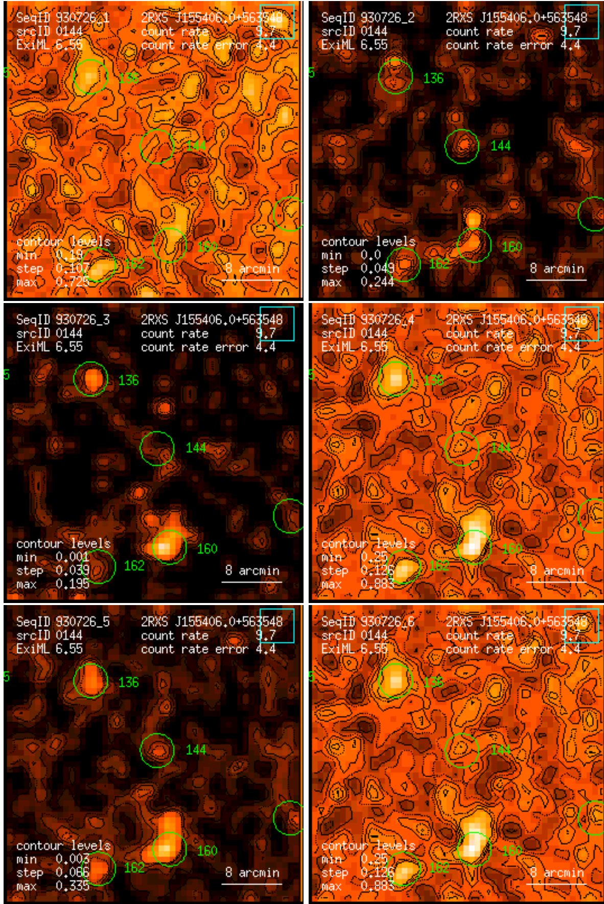
Figure 144: RASS 930726: detection 0144: band rate images, Gaussian filter: (1) PSPC channels 11 – 41, (2) 52 – 90, (3) 91 – 201, (4) 11 – 235, (5) 52 – 201, (6) 11 – 201. Broad band rates in counts/ks. Band rate contour levels in counts/ks/arcmin 2 .
