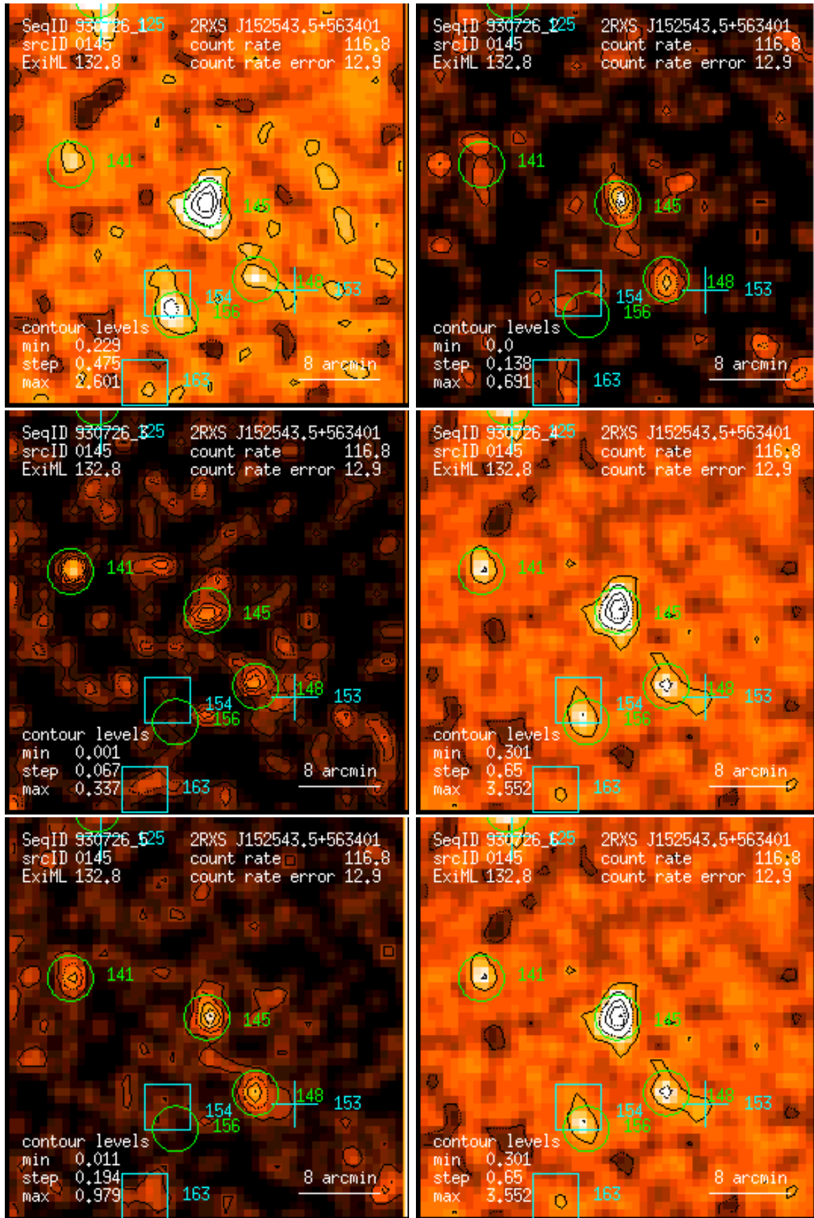
Figure 145: RASS 930726: detection 0145: band rate images, Gaussian filter: (1) PSPC channels 11 – 41, (2) 52 – 90, (3) 91 – 201, (4) 11 – 235, (5) 52 – 201, (6) 11 – 201. Broad band rates in counts/ks. Band rate contour levels in counts/ks/arcmin 2 .
