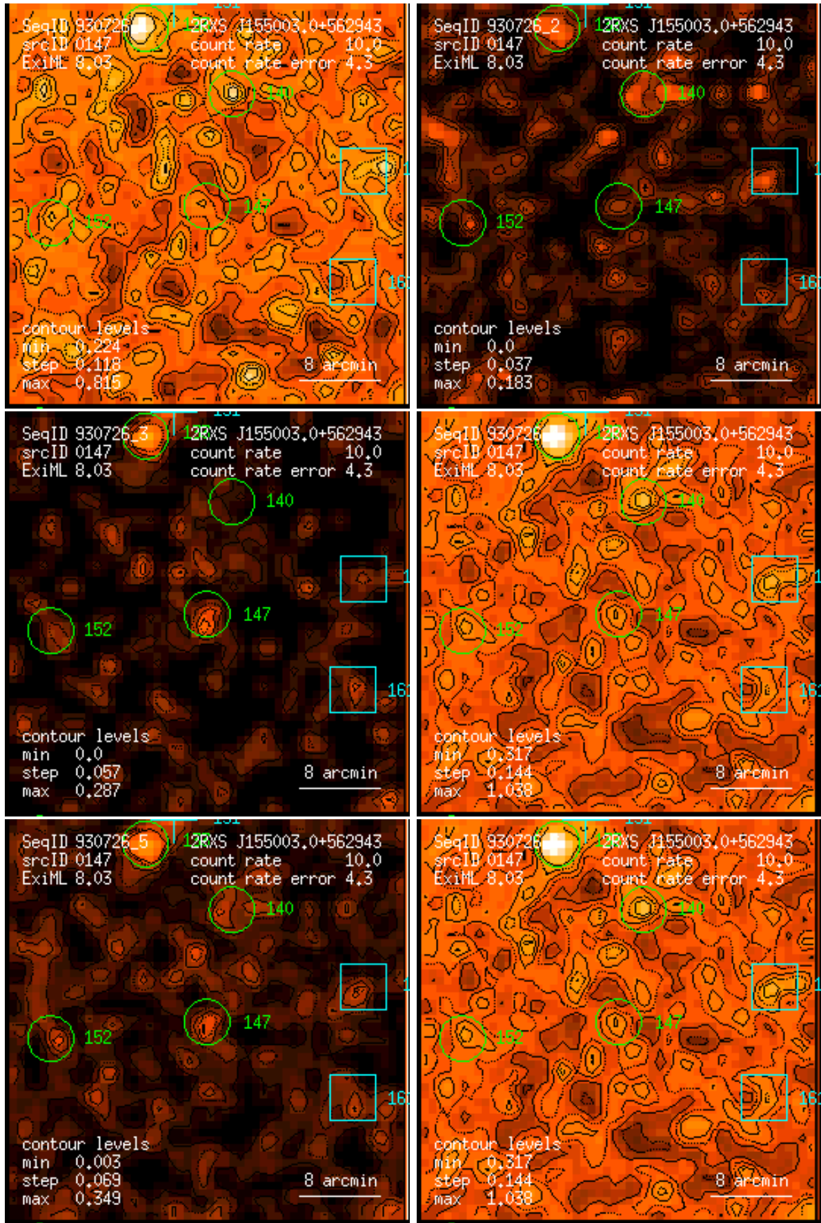
Figure 147: RASS 930726: detection 0147: band rate images, Gaussian filter: (1) PSPC channels 11 – 41, (2) 52 – 90, (3) 91 – 201, (4) 11 – 235, (5) 52 – 201, (6) 11 – 201. Broad band rates in counts/ks. Band rate contour levels in counts/ks/arcmin 2 .
