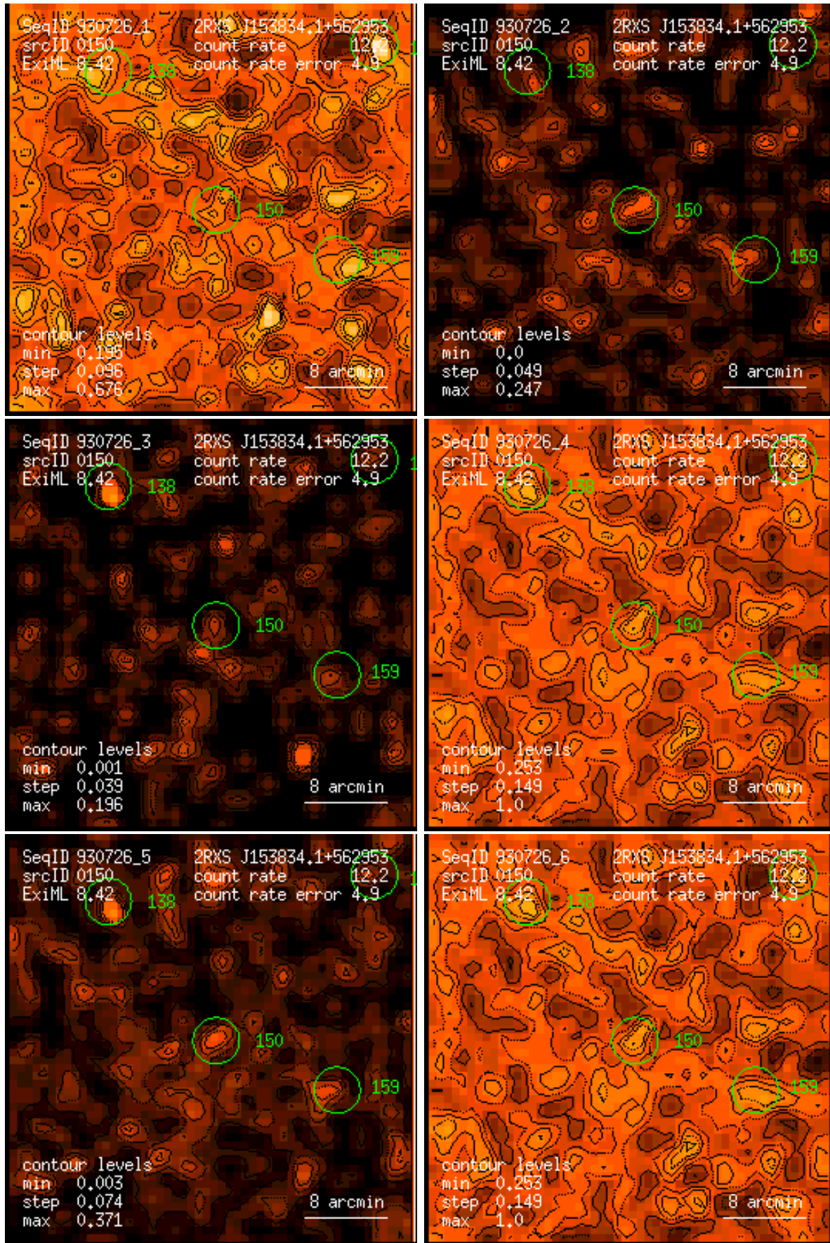
Figure 150: RASS 930726: detection 0150: band rate images, Gaussian filter: (1) PSPC channels 11 – 41, (2) 52 – 90, (3) 91 – 201, (4) 11 – 235, (5) 52 – 201, (6) 11 – 201. Broad band rates in counts/ks. Band rate contour levels in counts/ks/arcmin 2 .
