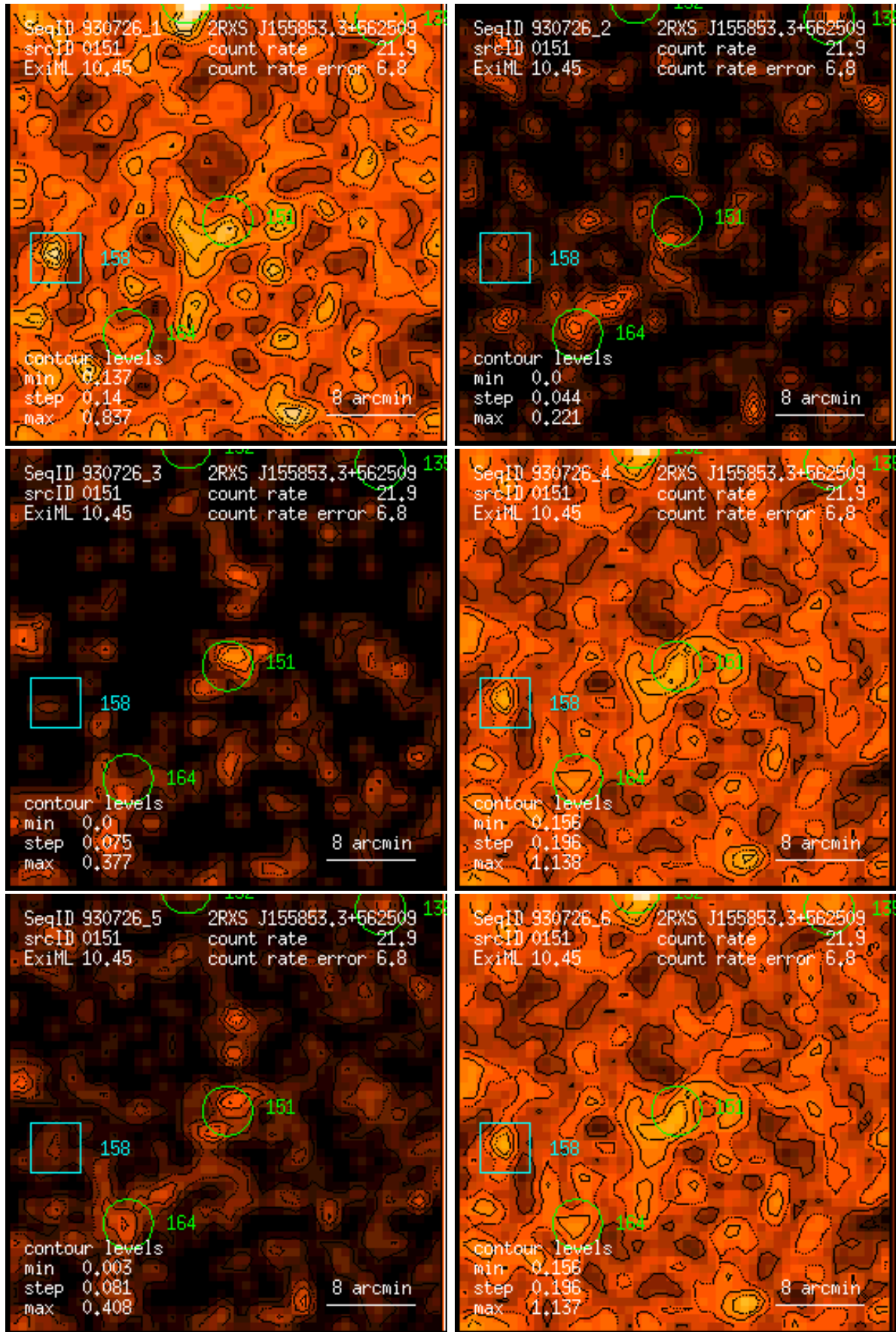
Figure 151: RASS 930726: detection 0151: band rate images, Gaussian filter: (1) PSPC channels 11 – 41, (2) 52 – 90, (3) 91 – 201, (4) 11 – 235, (5) 52 – 201, (6) 11 – 201. Broad band rates in counts/ks. Band rate contour levels in counts/ks/arcmin 2 .
