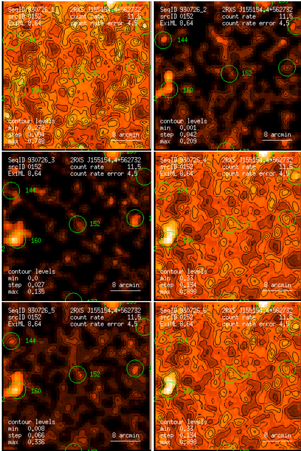
Figure 152: RASS 930726: detection 0152: band rate images, Gaussian filter: (1) PSPC channels 11 – 41, (2) 52 – 90, (3) 91 – 201, (4) 11 – 235, (5) 52 – 201, (6) 11 – 201. Broad band rates in counts/ks. Band rate contour levels in counts/ks/arcmin 2 .
