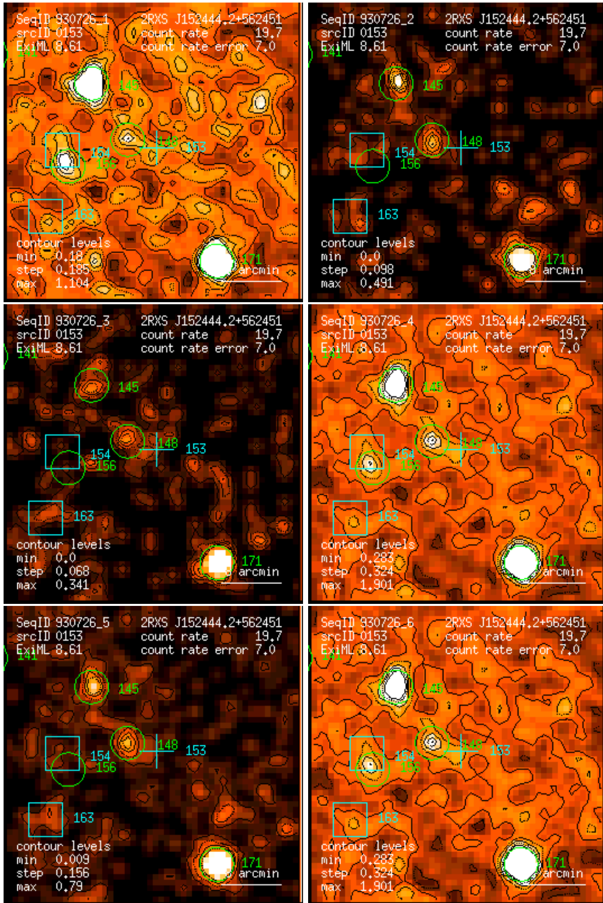
Figure 153: RASS 930726: detection 0153: band rate images, Gaussian filter: (1) PSPC channels 11 – 41, (2) 52 – 90, (3) 91 – 201, (4) 11 – 235, (5) 52 – 201, (6) 11 – 201. Broad band rates in counts/ks. Band rate contour levels in counts/ks/arcmin 2 .
