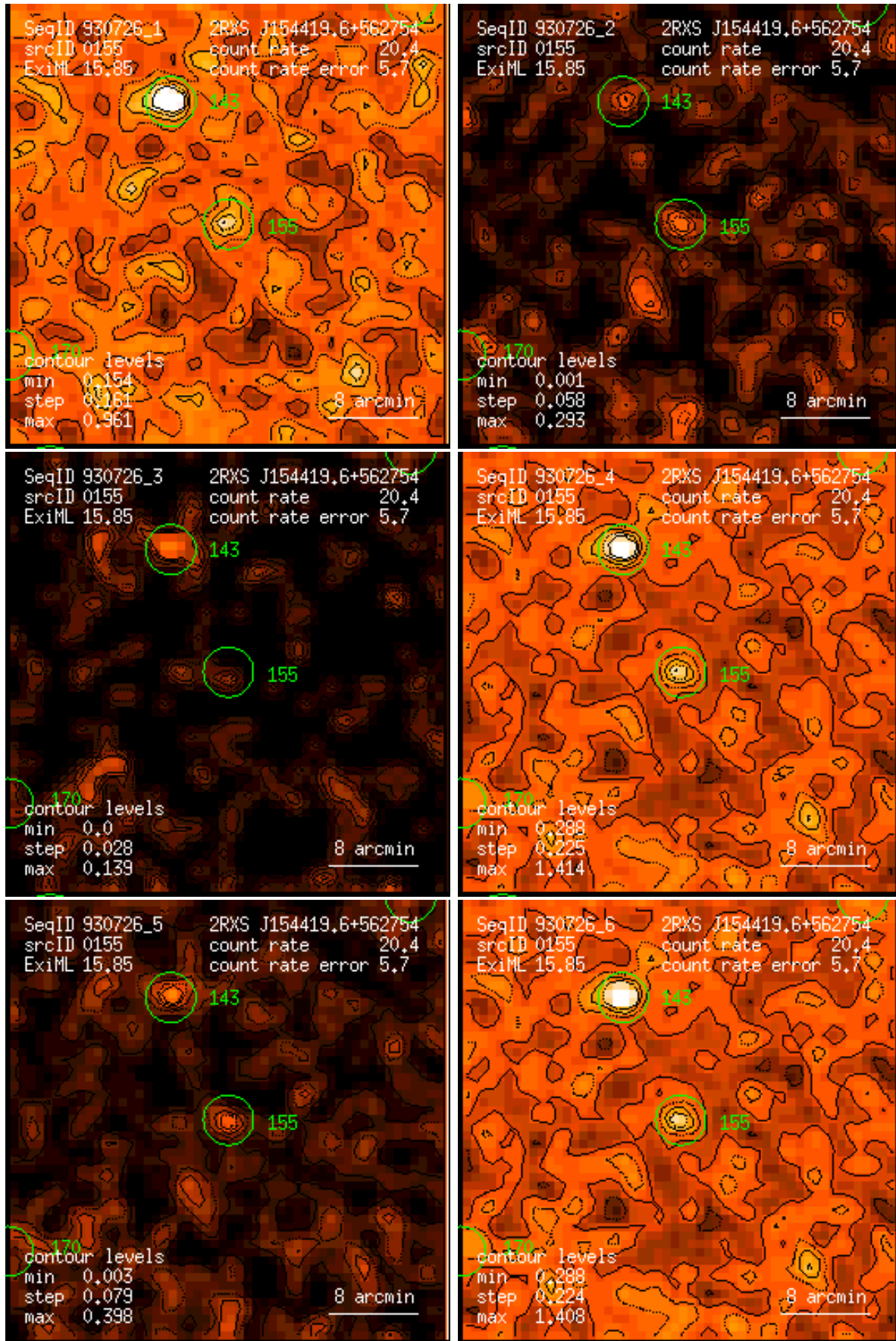
Figure 155: RASS 930726: detection 0155: band rate images, Gaussian filter: (1) PSPC channels 11 – 41, (2) 52 – 90, (3) 91 – 201, (4) 11 – 235, (5) 52 – 201, (6) 11 – 201. Broad band rates in counts/ks. Band rate contour levels in counts/ks/arcmin 2 .
