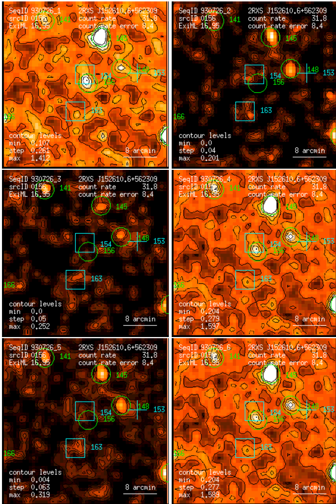
Figure 156: RASS 930726: detection 0156: band rate images, Gaussian filter: (1) PSPC channels 11 – 41, (2) 52 – 90, (3) 91 – 201, (4) 11 – 235, (5) 52 – 201, (6) 11 – 201. Broad band rates in counts/ks. Band rate contour levels in counts/ks/arcmin 2 .
