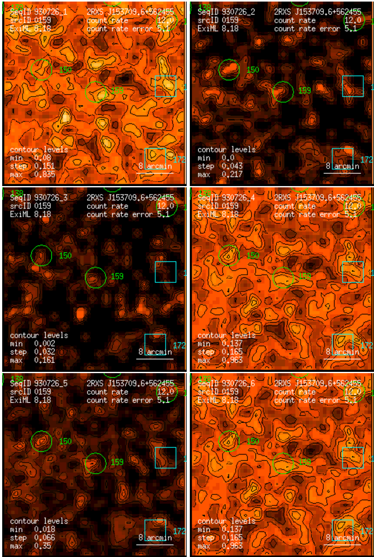
Figure 159: RASS 930726: detection 0159: band rate images, Gaussian filter: (1) PSPC channels 11 – 41, (2) 52 – 90, (3) 91 – 201, (4) 11 – 235, (5) 52 – 201, (6) 11 – 201. Broad band rates in counts/ks. Band rate contour levels in counts/ks/arcmin 2 .
