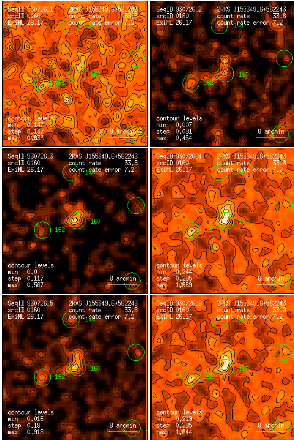
Figure 160: RASS 930726: detection 0160: band rate images, Gaussian filter: (1) PSPC channels 11 – 41, (2) 52 – 90, (3) 91 – 201, (4) 11 – 235, (5) 52 – 201, (6) 11 – 201. Broad band rates in counts/ks. Band rate contour levels in counts/ks/arcmin 2 .
