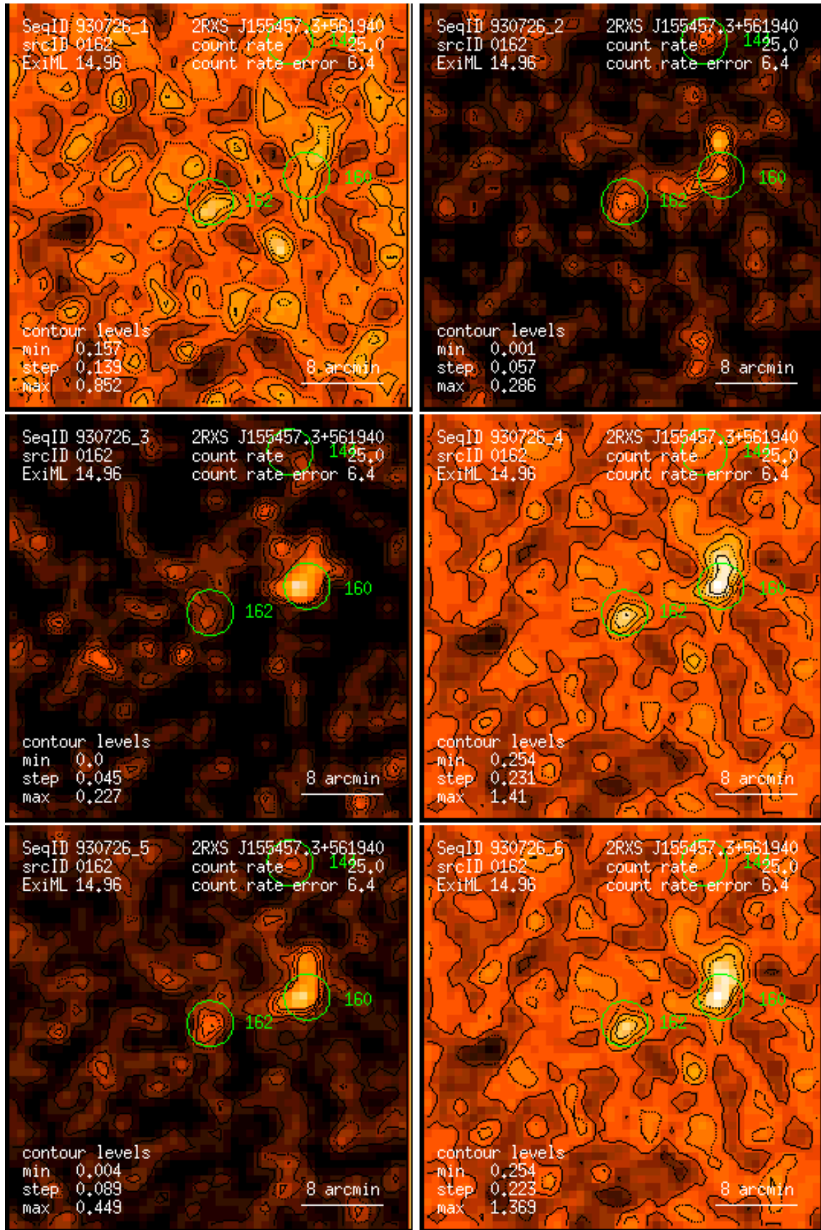
Figure 162: RASS 930726: detection 0162: band rate images, Gaussian filter: (1) PSPC channels 11 – 41, (2) 52 – 90, (3) 91 – 201, (4) 11 – 235, (5) 52 – 201, (6) 11 – 201. Broad band rates in counts/ks. Band rate contour levels in counts/ks/arcmin 2 .
