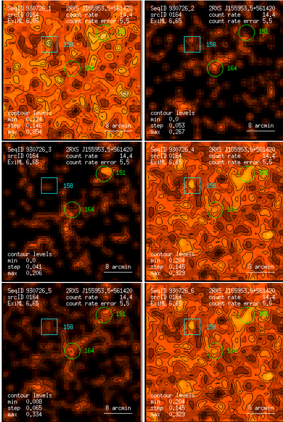
Figure 164: RASS 930726: detection 0164: band rate images, Gaussian filter: (1) PSPC channels 11 – 41, (2) 52 – 90, (3) 91 – 201, (4) 11 – 235, (5) 52 – 201, (6) 11 – 201. Broad band rates in counts/ks. Band rate contour levels in counts/ks/arcmin 2 .
