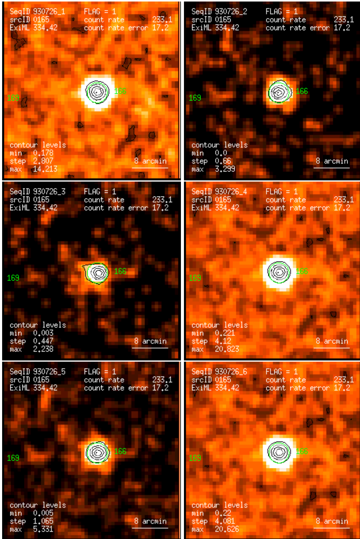
Figure 165: RASS 930726: detection 0165: band rate images, Gaussian filter: (1) PSPC channels 11 – 41, (2) 52 – 90, (3) 91 – 201, (4) 11 – 235, (5) 52 – 201, (6) 11 – 201. Broad band rates in counts/ks. Band rate contour levels in counts/ks/arcmin 2 .
