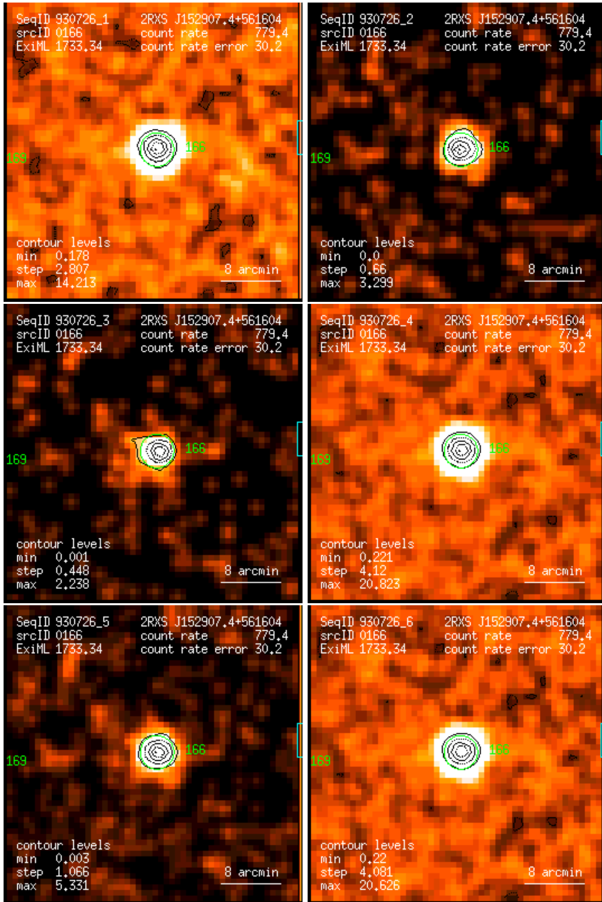
Figure 166: RASS 930726: detection 0166: band rate images, Gaussian filter: (1) PSPC channels 11 – 41, (2) 52 – 90, (3) 91 – 201, (4) 11 – 235, (5) 52 – 201, (6) 11 – 201. Broad band rates in counts/ks. Band rate contour levels in counts/ks/arcmin 2 .
