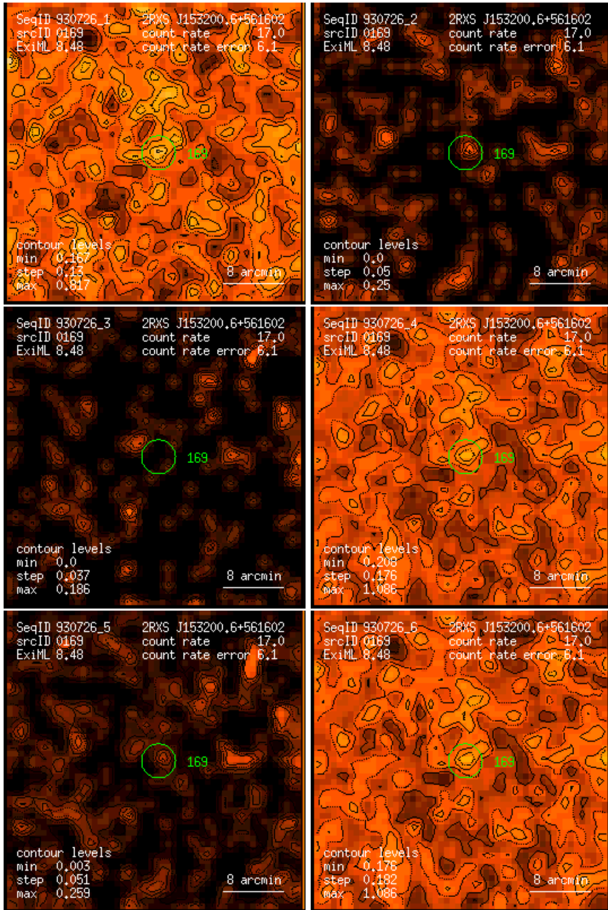
Figure 169: RASS 930726: detection 0169: band rate images, Gaussian filter: (1) PSPC channels 11 – 41, (2) 52 – 90, (3) 91 – 201, (4) 11 – 235, (5) 52 – 201, (6) 11 – 201. Broad band rates in counts/ks. Band rate contour levels in counts/ks/arcmin 2 .
