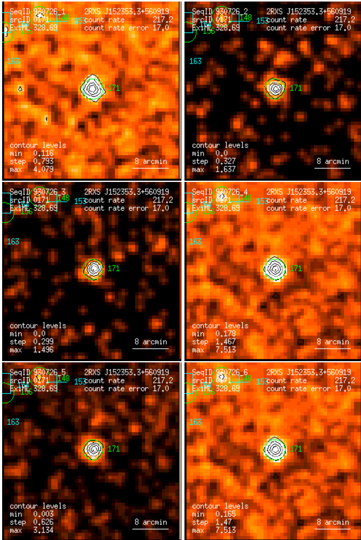
Figure 171: RASS 930726: detection 0171: band rate images, Gaussian filter: (1) PSPC channels 11 – 41, (2) 52 – 90, (3) 91 – 201, (4) 11 – 235, (5) 52 – 201, (6) 11 – 201. Broad band rates in counts/ks. Band rate contour levels in counts/ks/arcmin 2 .
