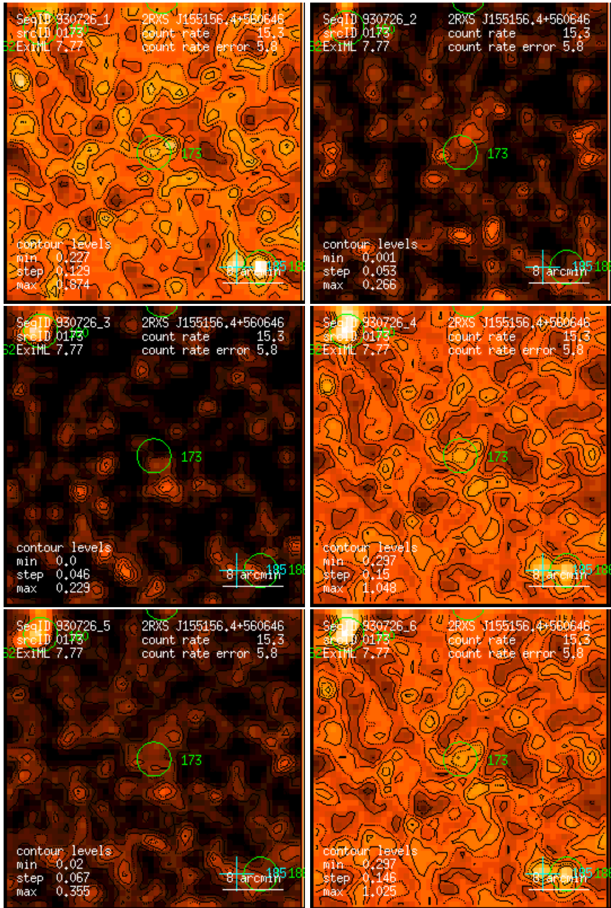
Figure 173: RASS 930726: detection 0173: band rate images, Gaussian filter: (1) PSPC channels 11 – 41, (2) 52 – 90, (3) 91 – 201, (4) 11 – 235, (5) 52 – 201, (6) 11 – 201. Broad band rates in counts/ks. Band rate contour levels in counts/ks/arcmin 2 .
