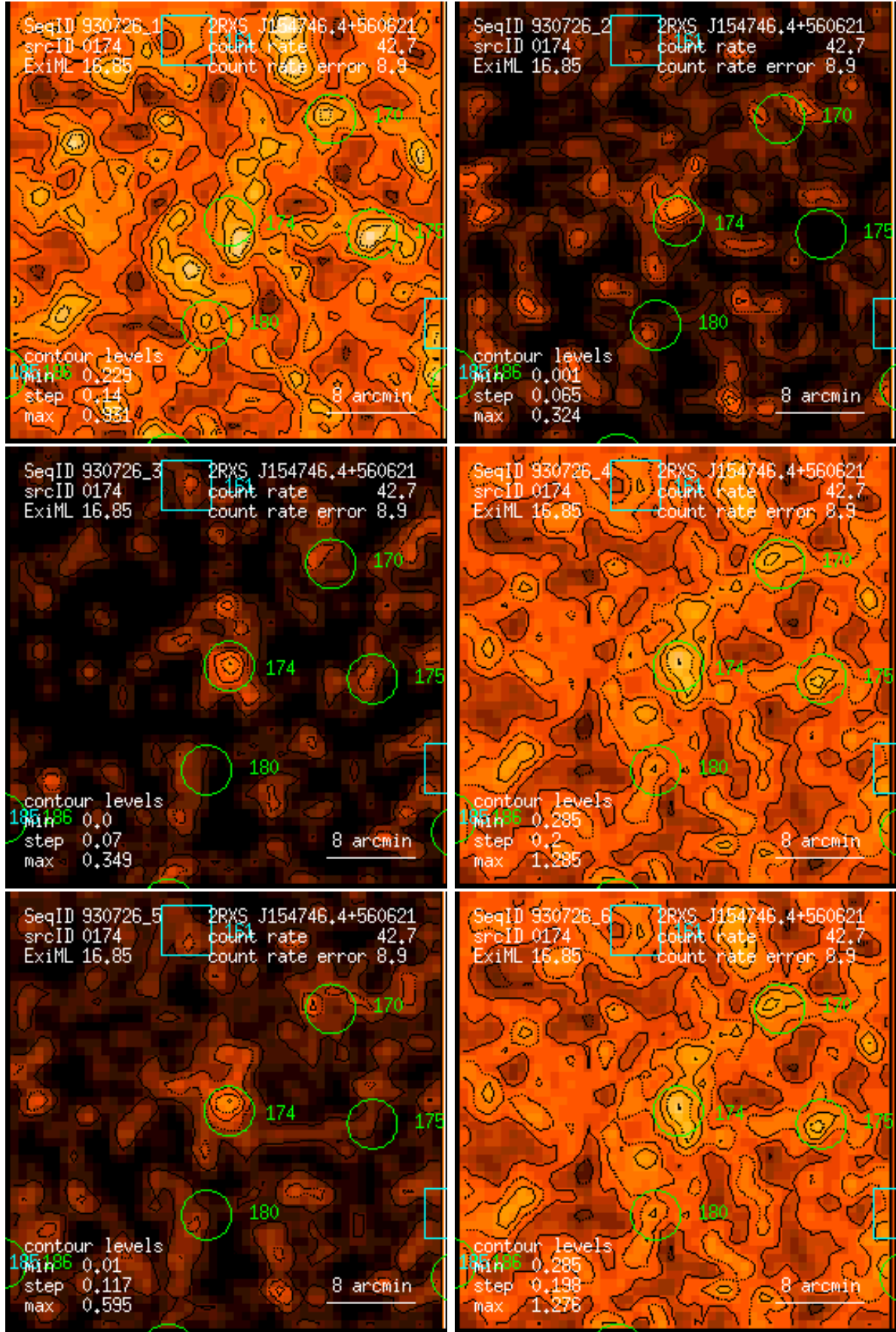
Figure 174: RASS 930726: detection 0174: band rate images, Gaussian filter: (1) PSPC channels 11 – 41, (2) 52 – 90, (3) 91 – 201, (4) 11 – 235, (5) 52 – 201, (6) 11 – 201. Broad band rates in counts/ks. Band rate contour levels in counts/ks/arcmin 2 .
