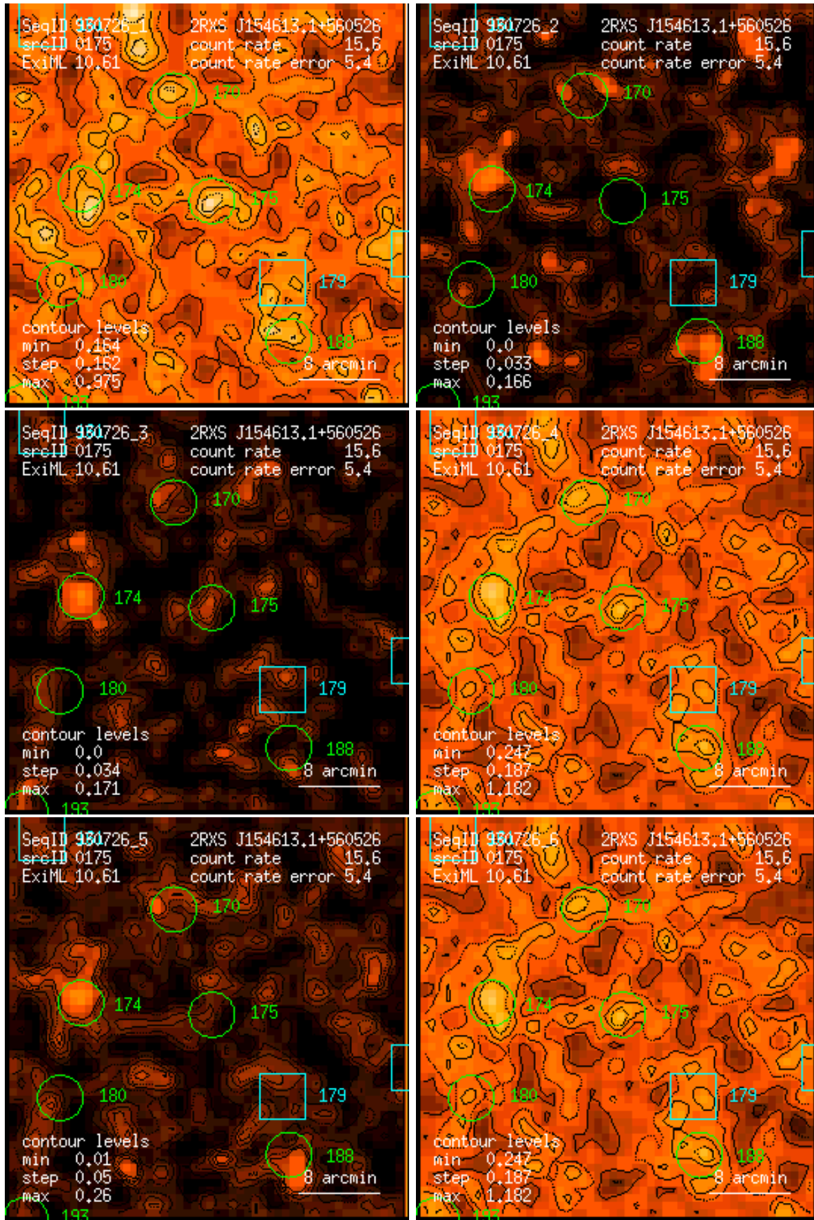
Figure 175: RASS 930726: detection 0175: band rate images, Gaussian filter: (1) PSPC channels 11 – 41, (2) 52 – 90, (3) 91 – 201, (4) 11 – 235, (5) 52 – 201, (6) 11 – 201. Broad band rates in counts/ks. Band rate contour levels in counts/ks/arcmin 2 .
