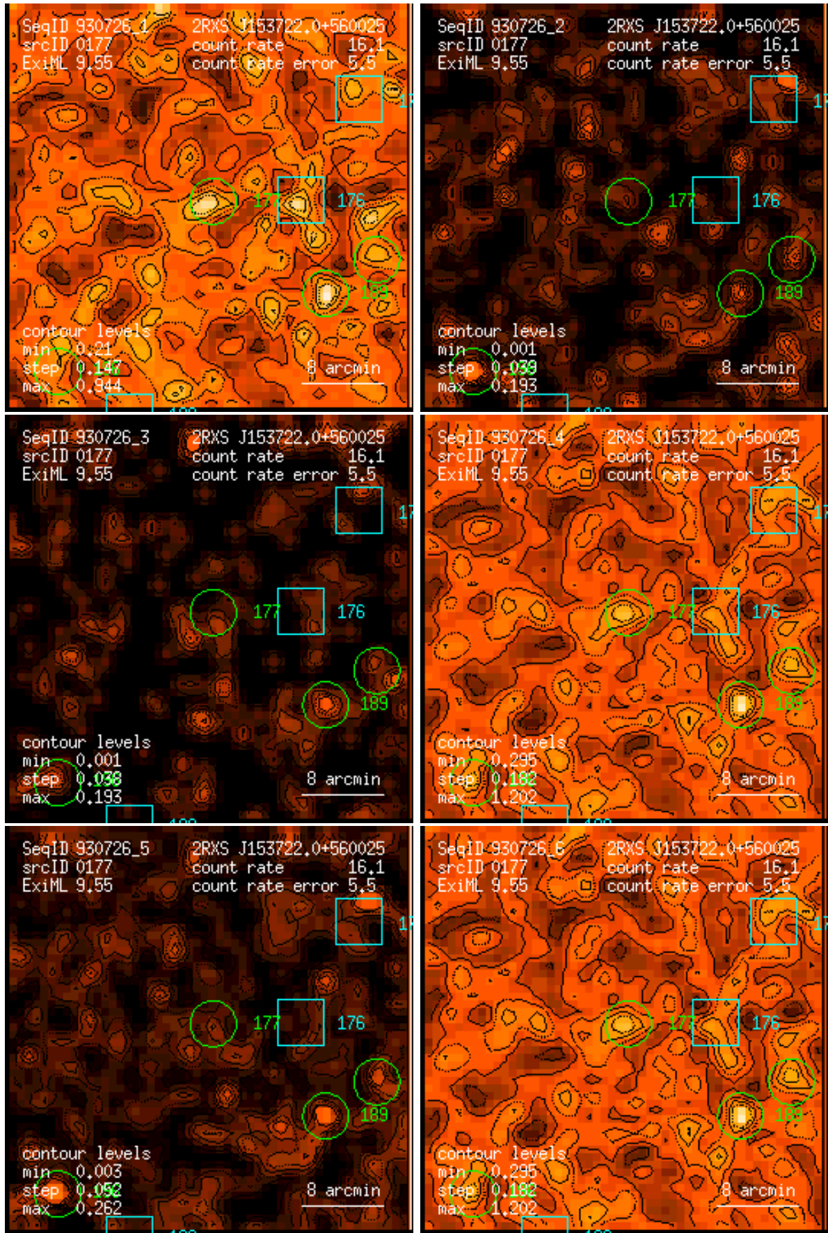
Figure 177: RASS 930726: detection 0177: band rate images, Gaussian filter: (1) PSPC channels 11 – 41, (2) 52 – 90, (3) 91 – 201, (4) 11 – 235, (5) 52 – 201, (6) 11 – 201. Broad band rates in counts/ks. Band rate contour levels in counts/ks/arcmin 2 .
