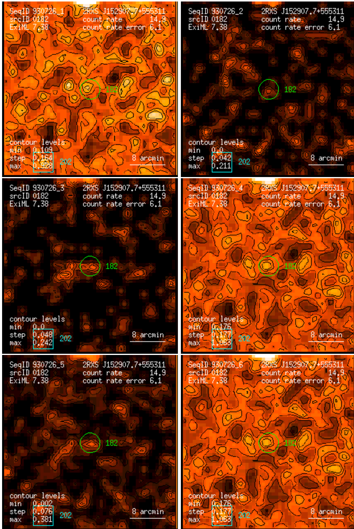
Figure 182: RASS 930726: detection 0182: band rate images, Gaussian filter: (1) PSPC channels 11 – 41, (2) 52 – 90, (3) 91 – 201, (4) 11 – 235, (5) 52 – 201, (6) 11 – 201. Broad band rates in counts/ks. Band rate contour levels in counts/ks/arcmin 2 .
