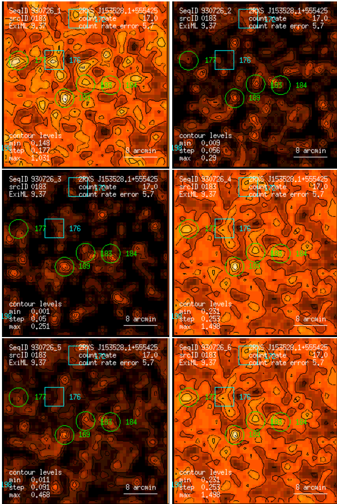
Figure 183: RASS 930726: detection 0183: band rate images, Gaussian filter: (1) PSPC channels 11 – 41, (2) 52 – 90, (3) 91 – 201, (4) 11 – 235, (5) 52 – 201, (6) 11 – 201. Broad band rates in counts/ks. Band rate contour levels in counts/ks/arcmin 2 .
