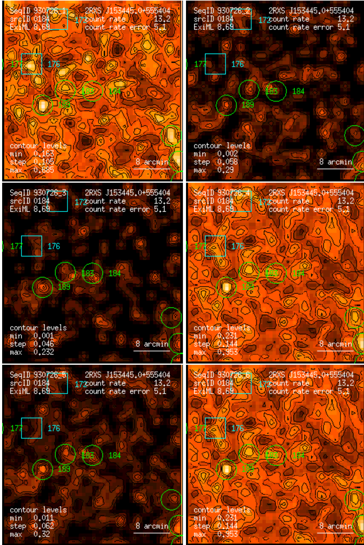
Figure 184: RASS 930726: detection 0184: band rate images, Gaussian filter: (1) PSPC channels 11 – 41, (2) 52 – 90, (3) 91 – 201, (4) 11 – 235, (5) 52 – 201, (6) 11 – 201. Broad band rates in counts/ks. Band rate contour levels in counts/ks/arcmin 2 .
