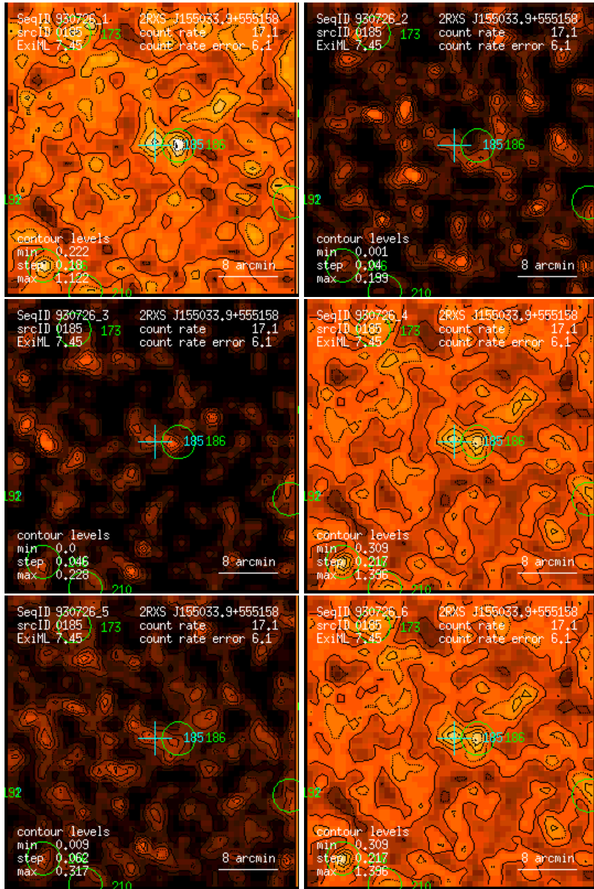
Figure 185: RASS 930726: detection 0185: band rate images, Gaussian filter: (1) PSPC channels 11 – 41, (2) 52 – 90, (3) 91 – 201, (4) 11 – 235, (5) 52 – 201, (6) 11 – 201. Broad band rates in counts/ks. Band rate contour levels in counts/ks/arcmin 2 .
