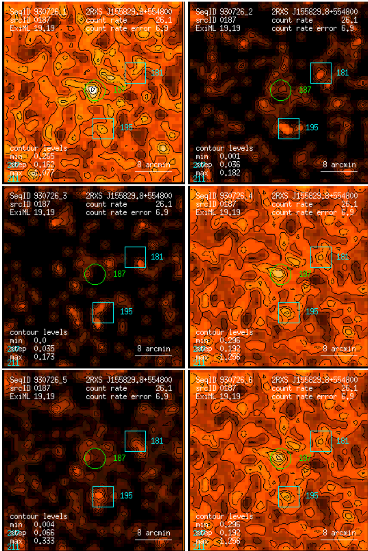
Figure 187: RASS 930726: detection 0187: band rate images, Gaussian filter: (1) PSPC channels 11 – 41, (2) 52 – 90, (3) 91 – 201, (4) 11 – 235, (5) 52 – 201, (6) 11 – 201. Broad band rates in counts/ks. Band rate contour levels in counts/ks/arcmin 2 .
