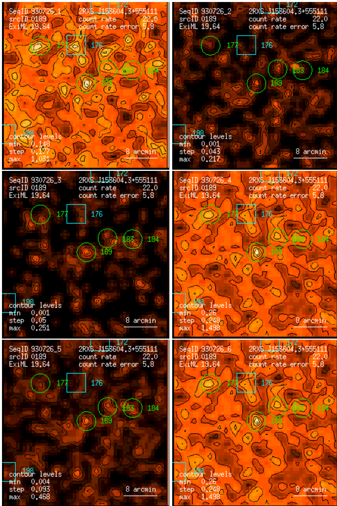
Figure 189: RASS 930726: detection 0189: band rate images, Gaussian filter: (1) PSPC channels 11 – 41, (2) 52 – 90, (3) 91 – 201, (4) 11 – 235, (5) 52 – 201, (6) 11 – 201. Broad band rates in counts/ks. Band rate contour levels in counts/ks/arcmin 2 .
