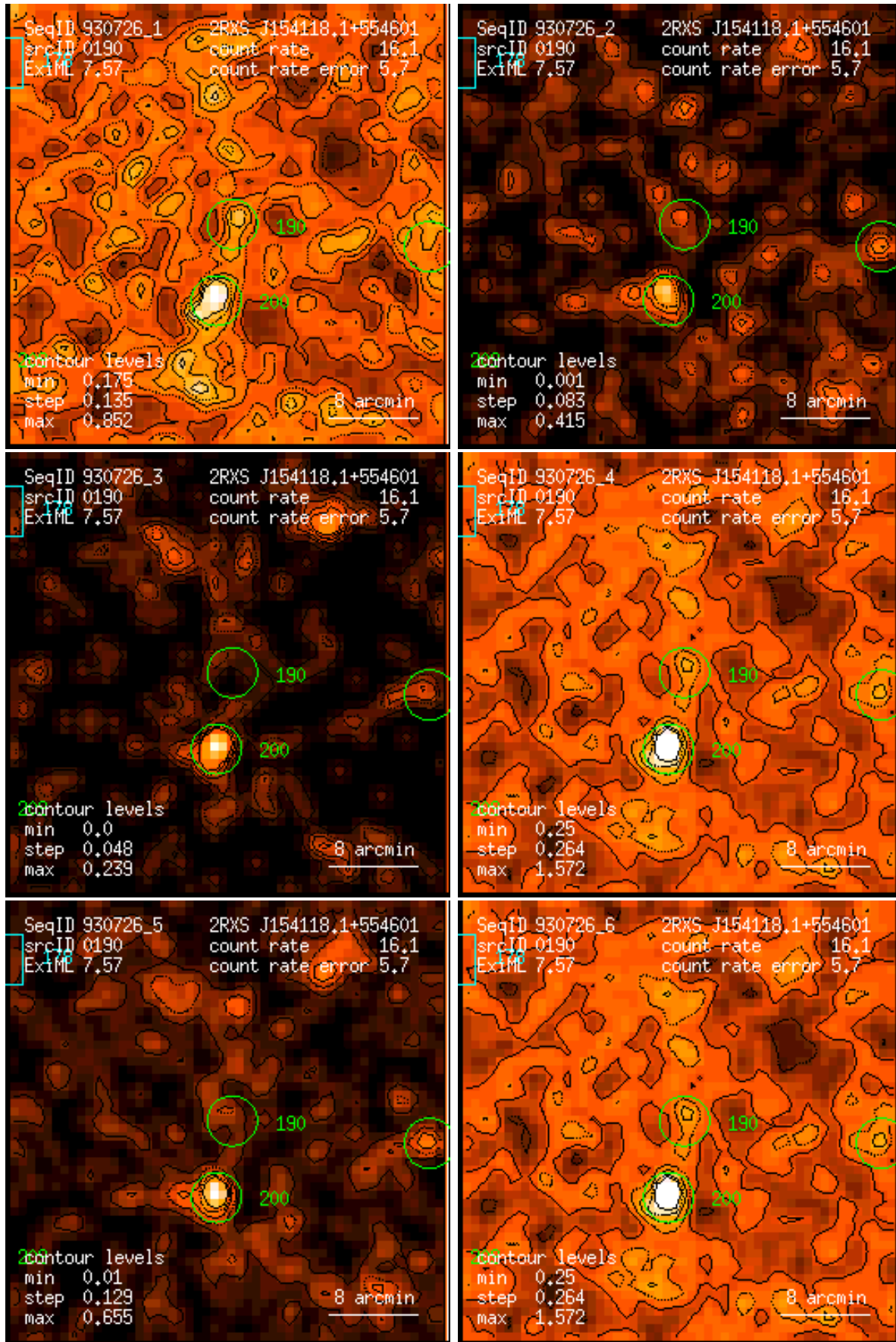
Figure 190: RASS 930726: detection 0190: band rate images, Gaussian filter: (1) PSPC channels 11 – 41, (2) 52 – 90, (3) 91 – 201, (4) 11 – 235, (5) 52 – 201, (6) 11 – 201. Broad band rates in counts/ks. Band rate contour levels in counts/ks/arcmin 2 .
