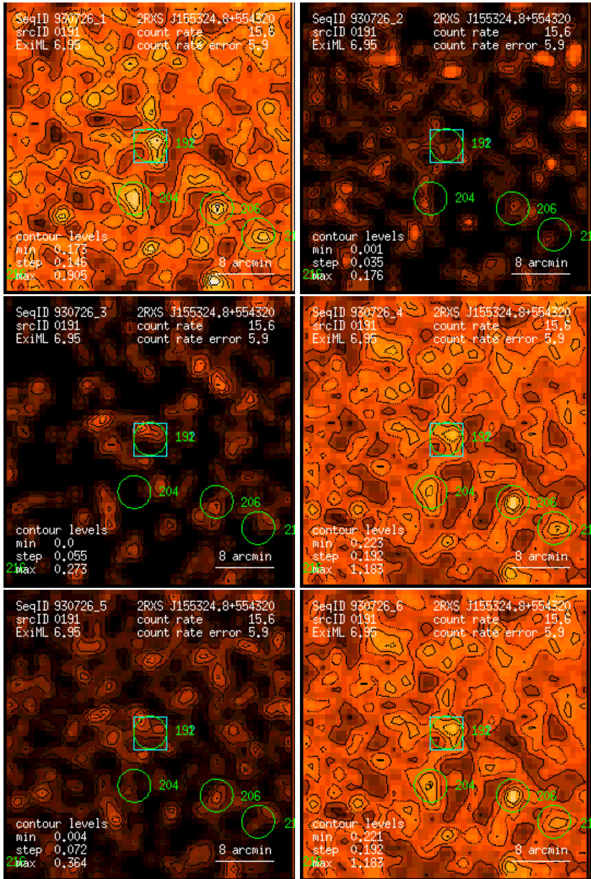
Figure 191: RASS 930726: detection 0191: band rate images, Gaussian filter: (1) PSPC channels 11 – 41, (2) 52 – 90, (3) 91 – 201, (4) 11 – 235, (5) 52 – 201, (6) 11 – 201. Broad band rates in counts/ks. Band rate contour levels in counts/ks/arcmin 2 .
