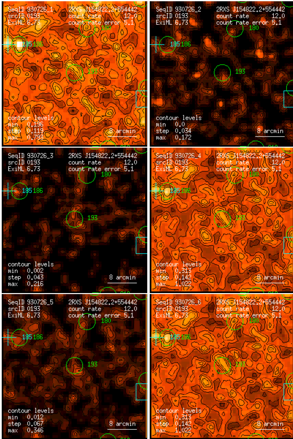
Figure 193: RASS 930726: detection 0193: band rate images, Gaussian filter: (1) PSPC channels 11 – 41, (2) 52 – 90, (3) 91 – 201, (4) 11 – 235, (5) 52 – 201, (6) 11 – 201. Broad band rates in counts/ks. Band rate contour levels in counts/ks/arcmin 2 .
